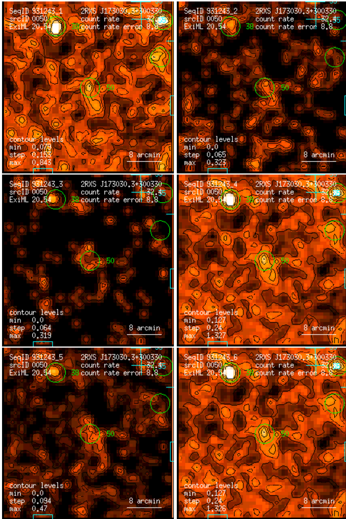
Figure 50: RASS 931243: detection 0050: band rate images, Gaussian filter: (1) PSPC channels 11 – 41, (2) 52 – 90, (3) 91 – 201, (4) 11 – 235, (5) 52 – 201, (6) 11 – 201. Broad band rates in counts/ks. Band rate contour levels in counts/ks/arcmin 2 .
