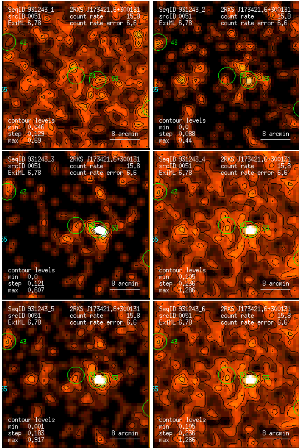
Figure 51: RASS 931243: detection 0051: band rate images, Gaussian filter: (1) PSPC channels 11 – 41, (2) 52 – 90, (3) 91 – 201, (4) 11 – 235, (5) 52 – 201, (6) 11 – 201. Broad band rates in counts/ks. Band rate contour levels in counts/ks/arcmin 2 .
