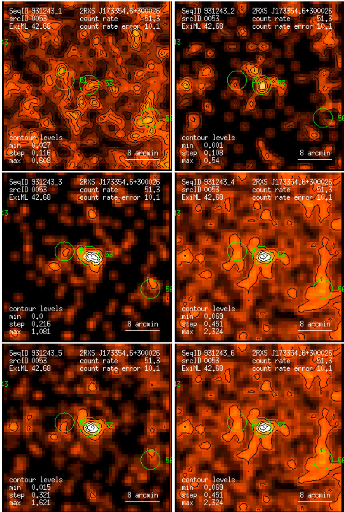
Figure 53: RASS 931243: detection 0053: band rate images, Gaussian filter: (1) PSPC channels 11 – 41, (2) 52 – 90, (3) 91 – 201, (4) 11 – 235, (5) 52 – 201, (6) 11 – 201. Broad band rates in counts/ks. Band rate contour levels in counts/ks/arcmin 2 .
