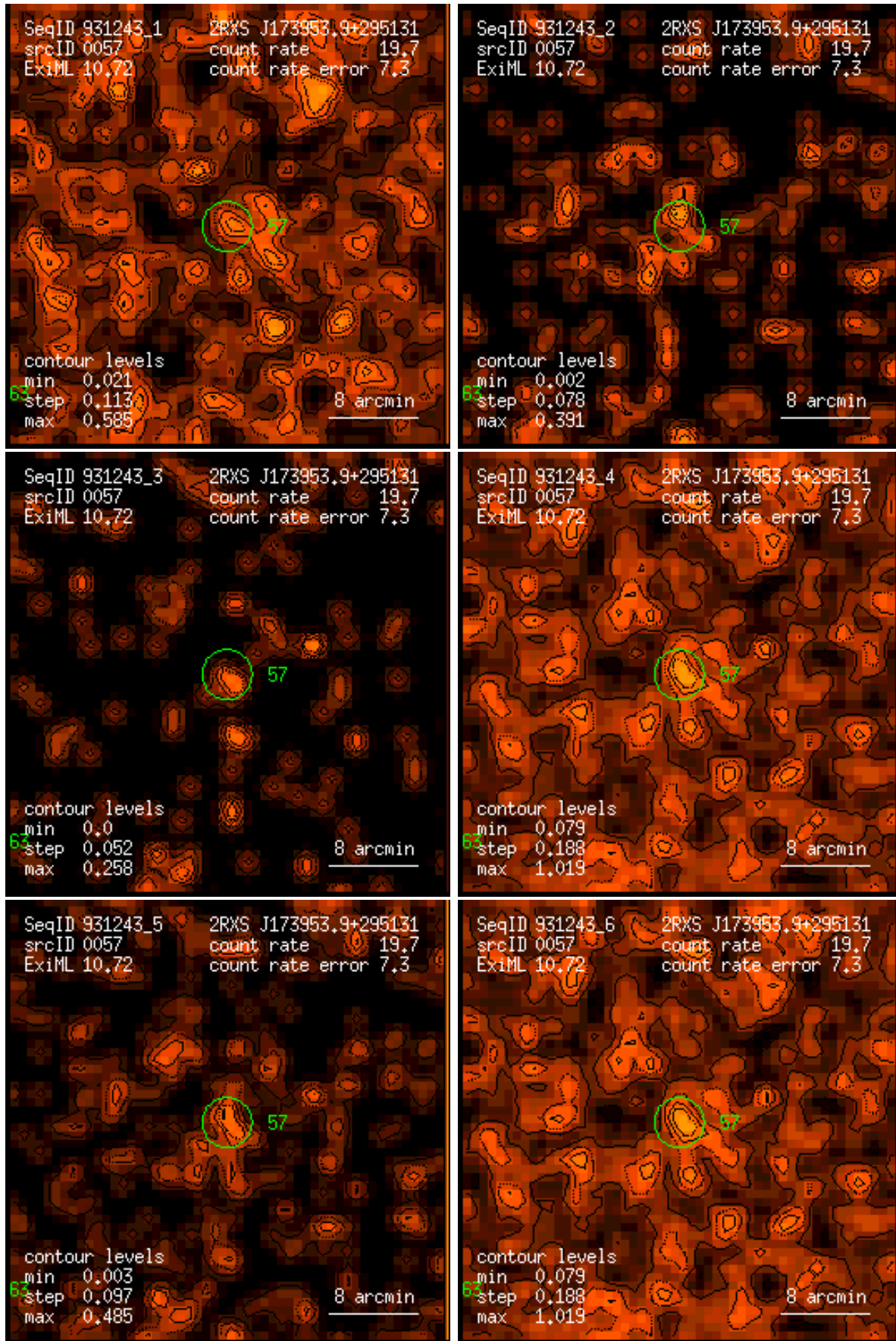
Figure 57: RASS 931243: detection 0057: band rate images, Gaussian filter: (1) PSPC channels 11 – 41, (2) 52 – 90, (3) 91 – 201, (4) 11 – 235, (5) 52 – 201, (6) 11 – 201. Broad band rates in counts/ks. Band rate contour levels in counts/ks/arcmin 2 .
