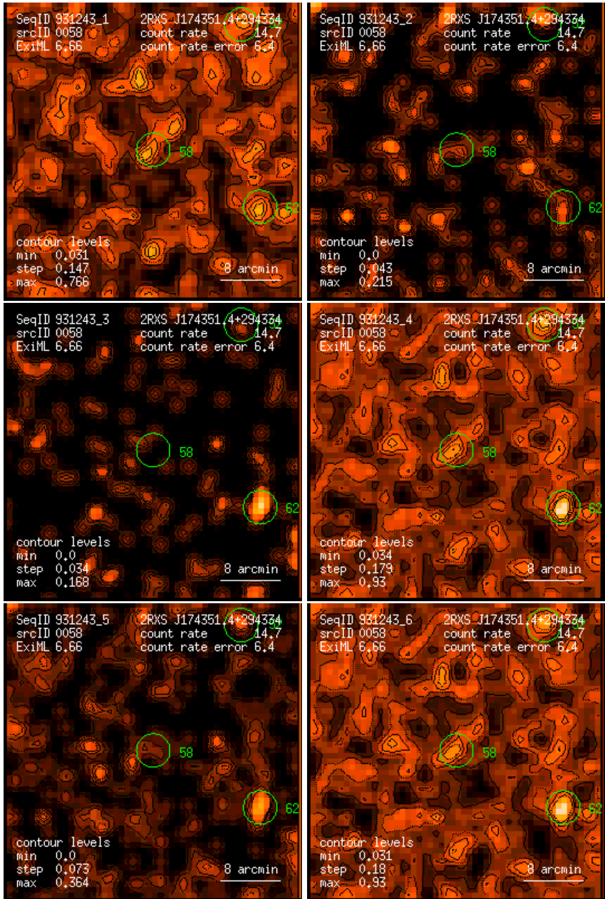
Figure 58: RASS 931243: detection 0058: band rate images, Gaussian filter: (1) PSPC channels 11 – 41, (2) 52 – 90, (3) 91 – 201, (4) 11 – 235, (5) 52 – 201, (6) 11 – 201. Broad band rates in counts/ks. Band rate contour levels in counts/ks/arcmin 2 .
