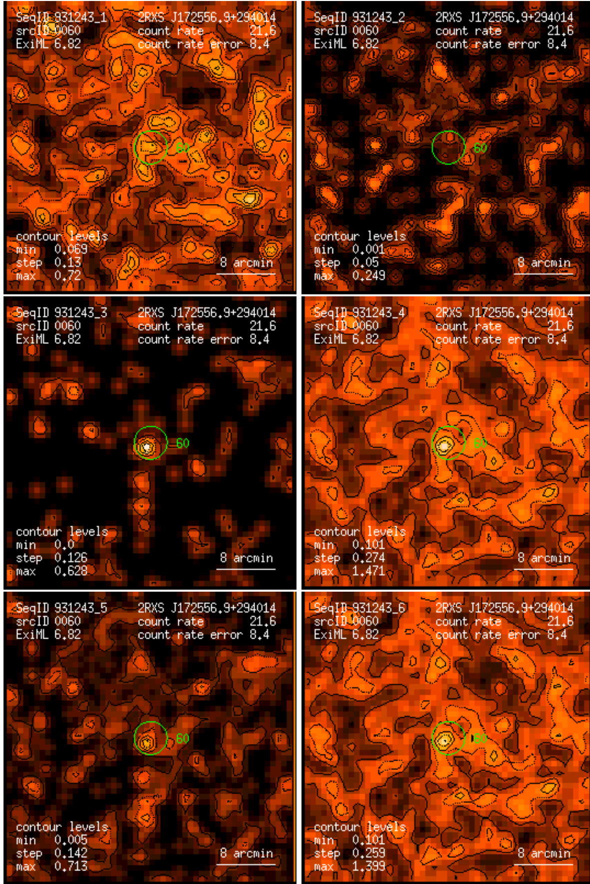
Figure 60: RASS 931243: detection 0060: band rate images, Gaussian filter: (1) PSPC channels 11 – 41, (2) 52 – 90, (3) 91 – 201, (4) 11 – 235, (5) 52 – 201, (6) 11 – 201. Broad band rates in counts/ks. Band rate contour levels in counts/ks/arcmin 2 .
