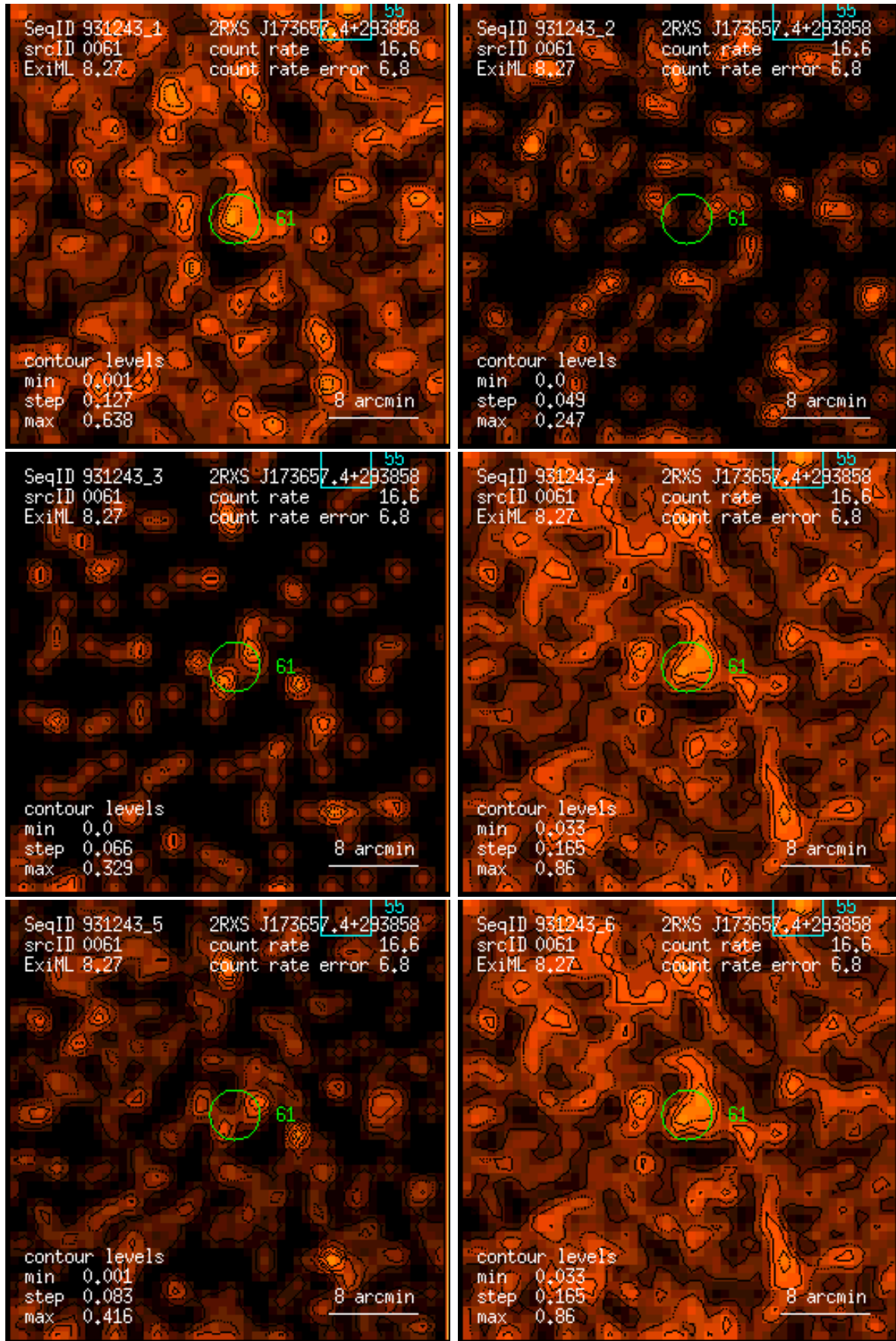
Figure 61: RASS 931243: detection 0061: band rate images, Gaussian filter: (1) PSPC channels 11 – 41, (2) 52 – 90, (3) 91 – 201, (4) 11 – 235, (5) 52 – 201, (6) 11 – 201. Broad band rates in counts/ks. Band rate contour levels in counts/ks/arcmin 2 .
