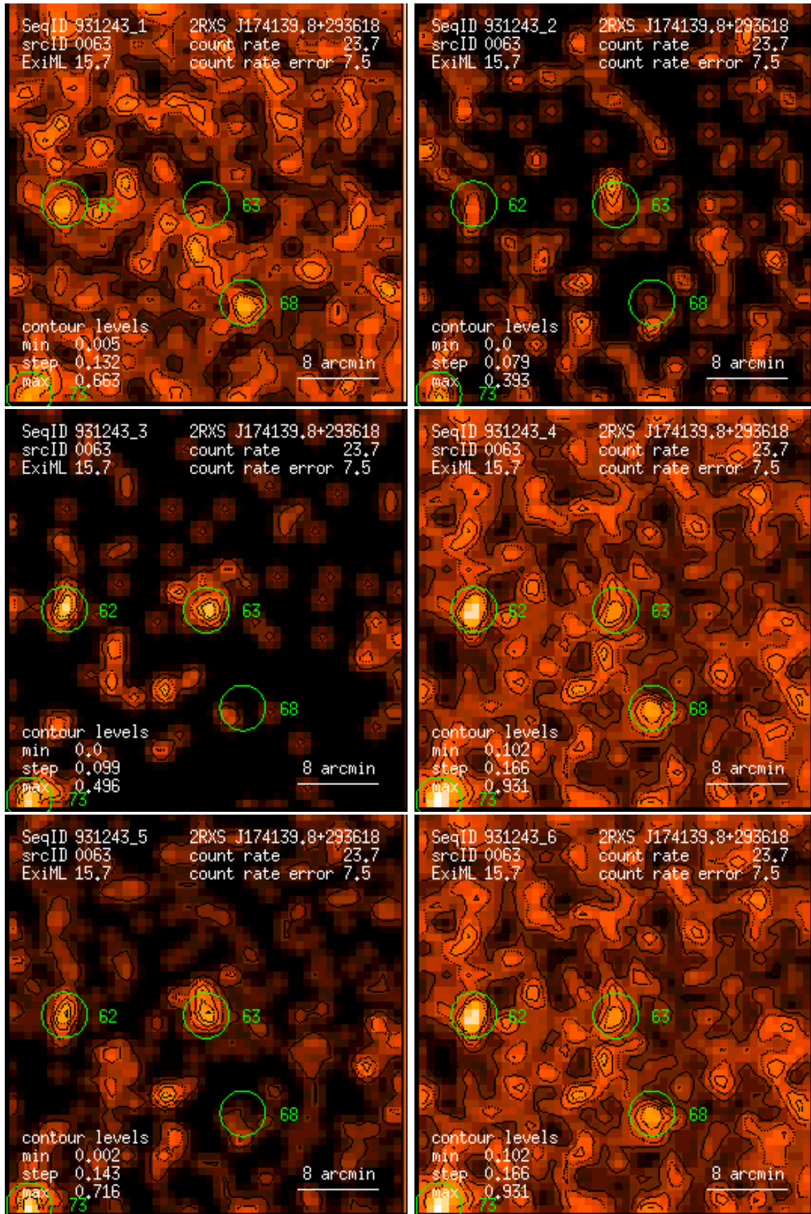
Figure 63: RASS 931243: detection 0063: band rate images, Gaussian filter: (1) PSPC channels 11 – 41, (2) 52 – 90, (3) 91 – 201, (4) 11 – 235, (5) 52 – 201, (6) 11 – 201. Broad band rates in counts/ks. Band rate contour levels in counts/ks/arcmin 2 .
