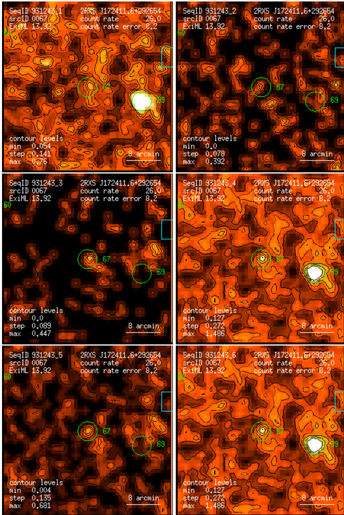
Figure 67: RASS 931243: detection 0067: band rate images, Gaussian filter: (1) PSPC channels 11 – 41, (2) 52 – 90, (3) 91 – 201, (4) 11 – 235, (5) 52 – 201, (6) 11 – 201. Broad band rates in counts/ks. Band rate contour levels in counts/ks/arcmin 2 .
