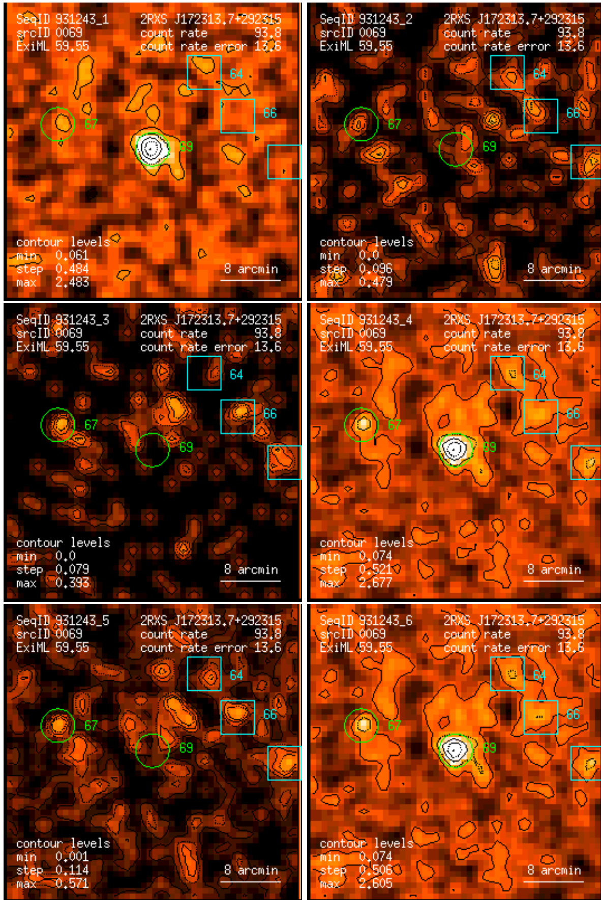
Figure 69: RASS 931243: detection 0069: band rate images, Gaussian filter: (1) PSPC channels 11 – 41, (2) 52 – 90, (3) 91 – 201, (4) 11 – 235, (5) 52 – 201, (6) 11 – 201. Broad band rates in counts/ks. Band rate contour levels in counts/ks/arcmin 2 .
