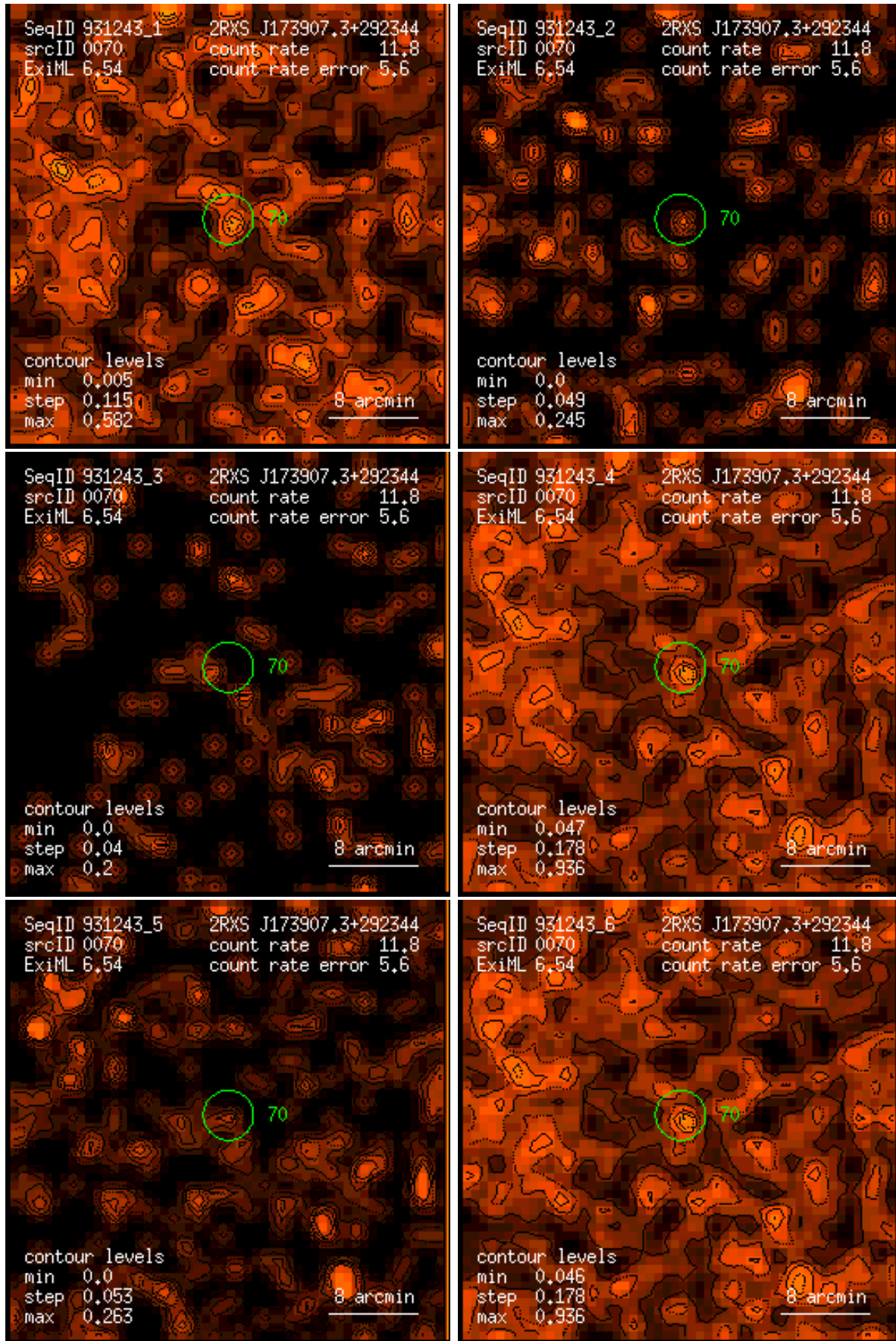
Figure 70: RASS 931243: detection 0070: band rate images, Gaussian filter: (1) PSPC channels 11 – 41, (2) 52 – 90, (3) 91 – 201, (4) 11 – 235, (5) 52 – 201, (6) 11 – 201. Broad band rates in counts/ks. Band rate contour levels in counts/ks/arcmin 2 .
