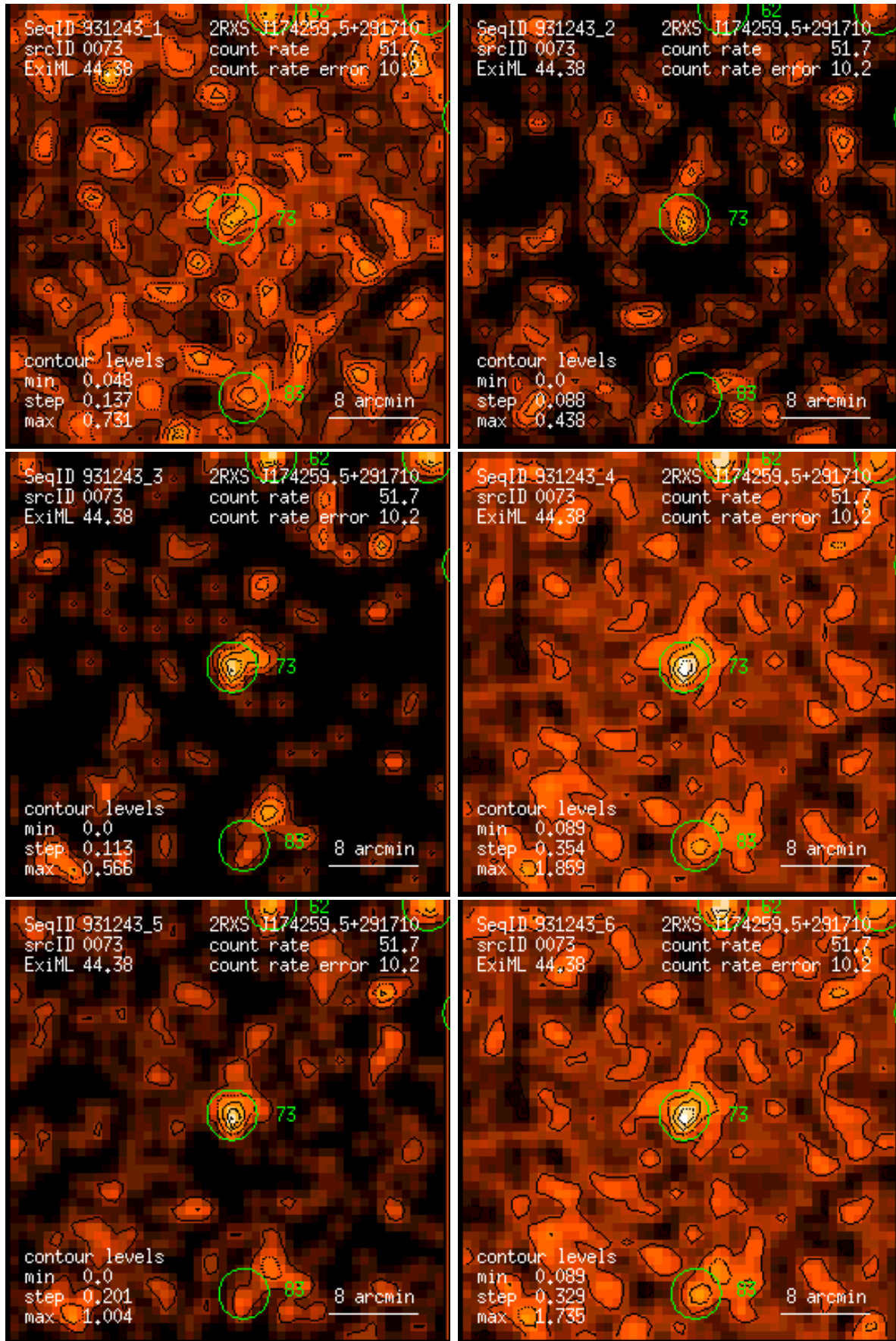
Figure 73: RASS 931243: detection 0073: band rate images, Gaussian filter: (1) PSPC channels 11 – 41, (2) 52 – 90, (3) 91 – 201, (4) 11 – 235, (5) 52 – 201, (6) 11 – 201. Broad band rates in counts/ks. Band rate contour levels in counts/ks/arcmin 2 .
