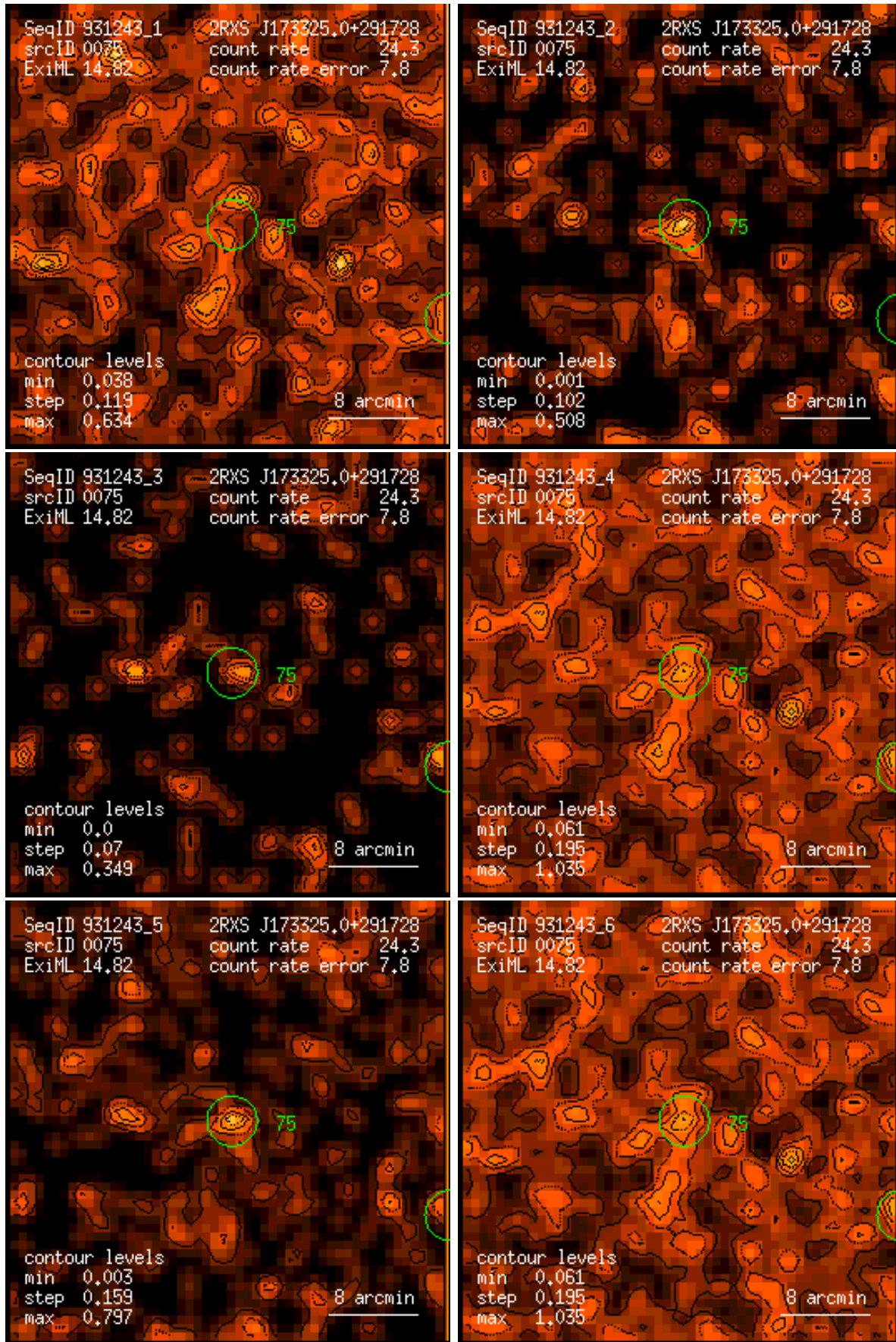
Figure 75: RASS 931243: detection 0075: band rate images, Gaussian filter: (1) PSPC channels 11 – 41, (2) 52 – 90, (3) 91 – 201, (4) 11 – 235, (5) 52 – 201, (6) 11 – 201. Broad band rates in counts/ks. Band rate contour levels in counts/ks/arcmin 2 .
