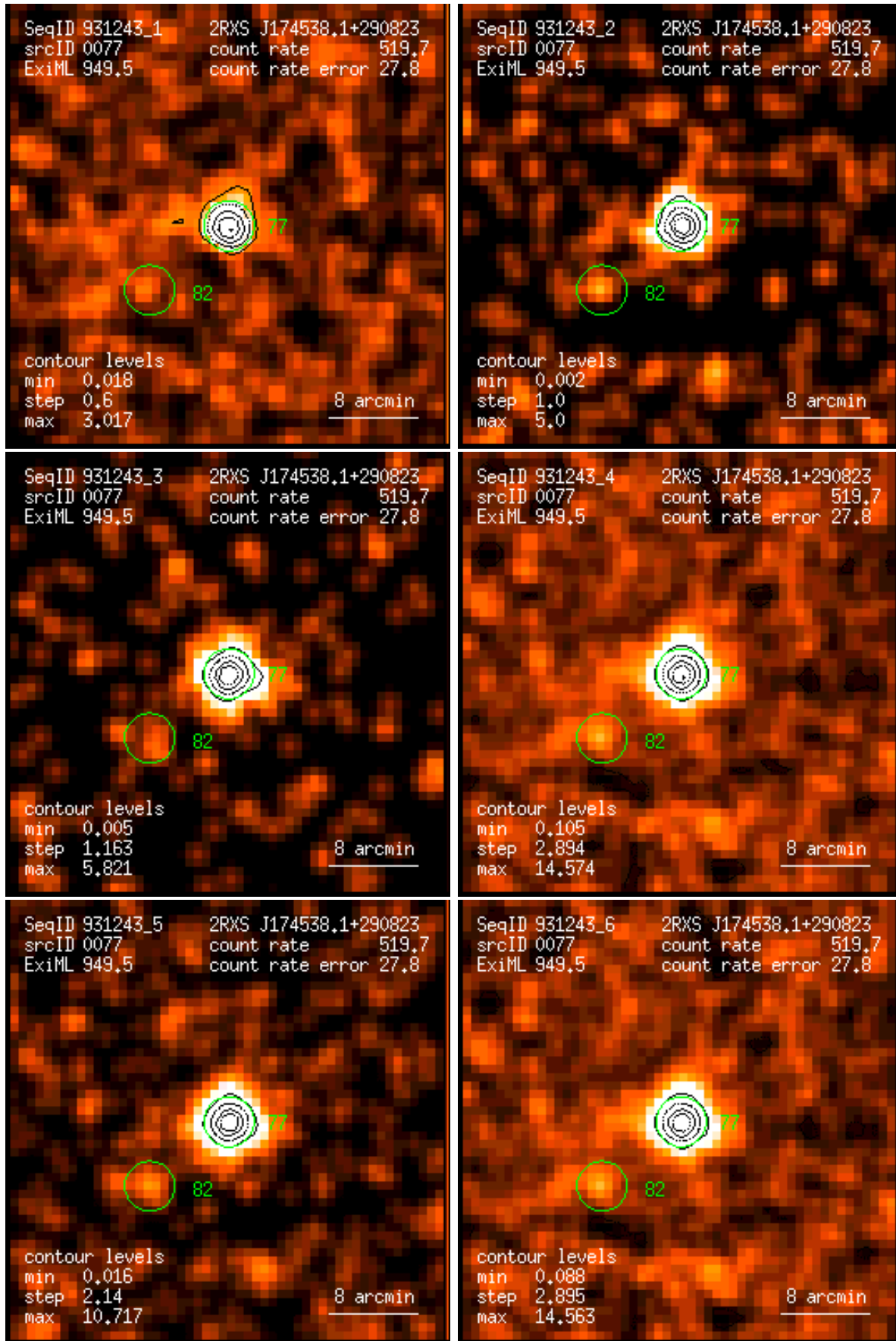
Figure 77: RASS 931243: detection 0077: band rate images, Gaussian filter: (1) PSPC channels 11 – 41, (2) 52 – 90, (3) 91 – 201, (4) 11 – 235, (5) 52 – 201, (6) 11 – 201. Broad band rates in counts/ks. Band rate contour levels in counts/ks/arcmin 2 .
