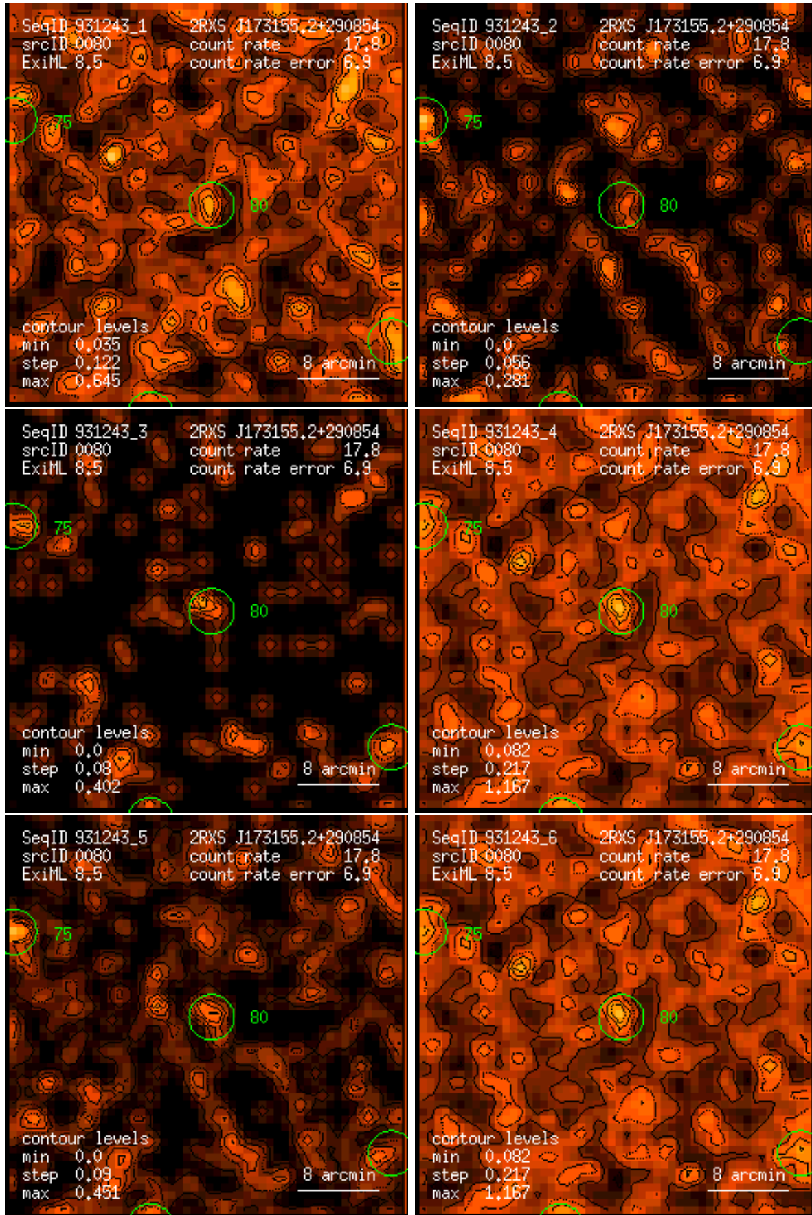
Figure 80: RASS 931243: detection 0080: band rate images, Gaussian filter: (1) PSPC channels 11 – 41, (2) 52 – 90, (3) 91 – 201, (4) 11 – 235, (5) 52 – 201, (6) 11 – 201. Broad band rates in counts/ks. Band rate contour levels in counts/ks/arcmin 2 .
