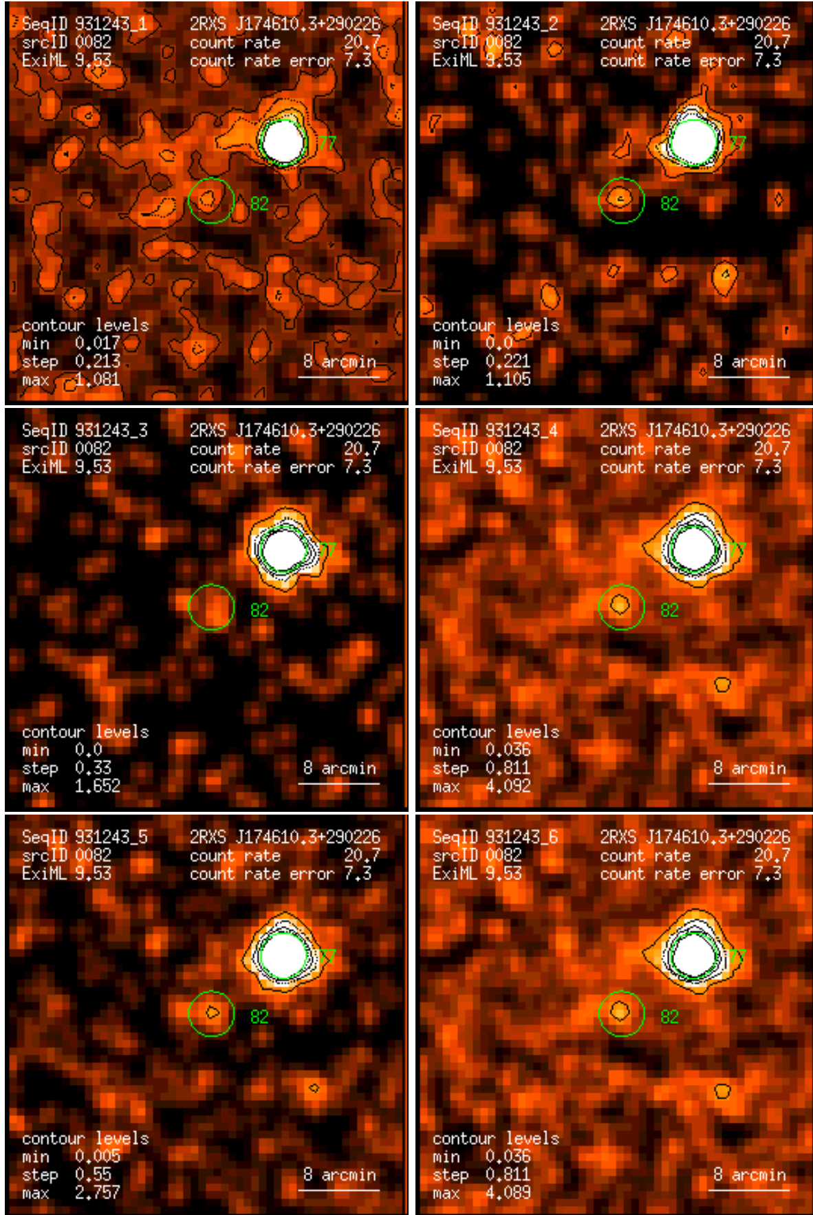
Figure 82: RASS 931243: detection 0082: band rate images, Gaussian filter: (1) PSPC channels 11 – 41, (2) 52 – 90, (3) 91 – 201, (4) 11 – 235, (5) 52 – 201, (6) 11 – 201. Broad band rates in counts/ks. Band rate contour levels in counts/ks/arcmin 2 .
