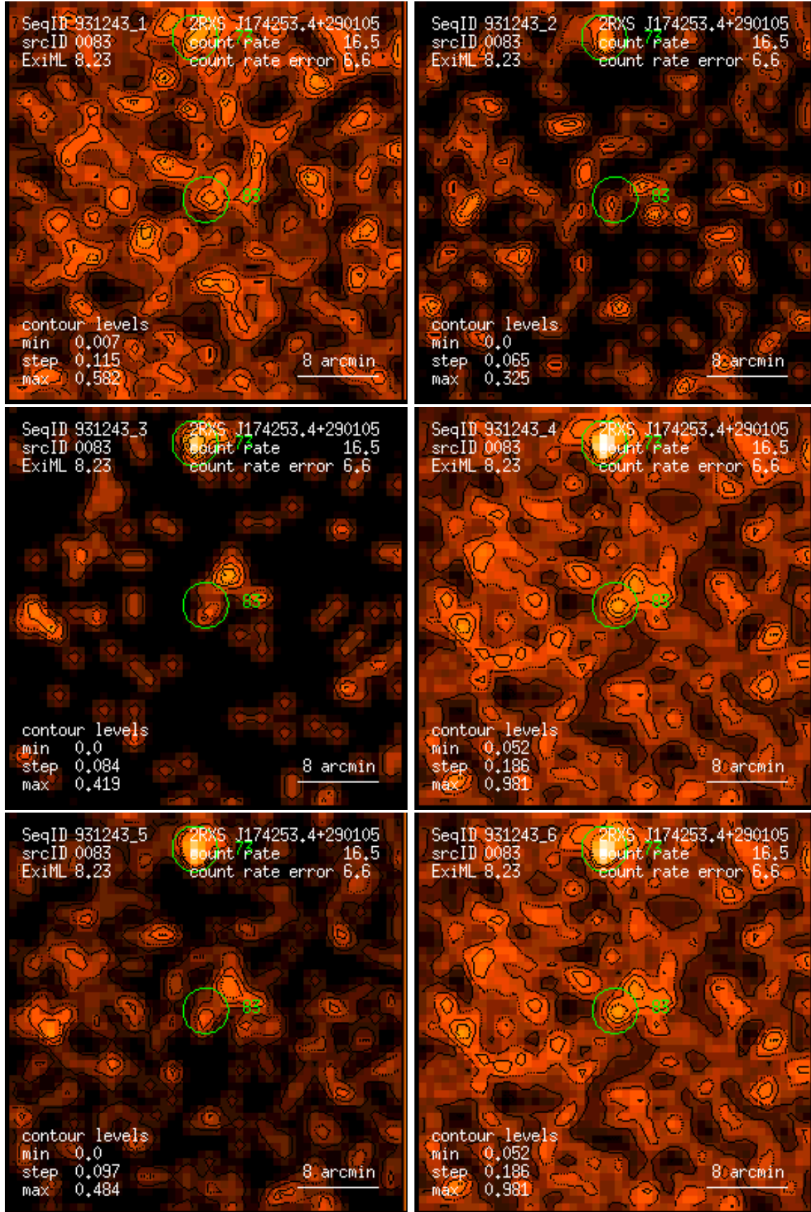
Figure 83: RASS 931243: detection 0083: band rate images, Gaussian filter: (1) PSPC channels 11 – 41, (2) 52 – 90, (3) 91 – 201, (4) 11 – 235, (5) 52 – 201, (6) 11 – 201. Broad band rates in counts/ks. Band rate contour levels in counts/ks/arcmin 2 .
