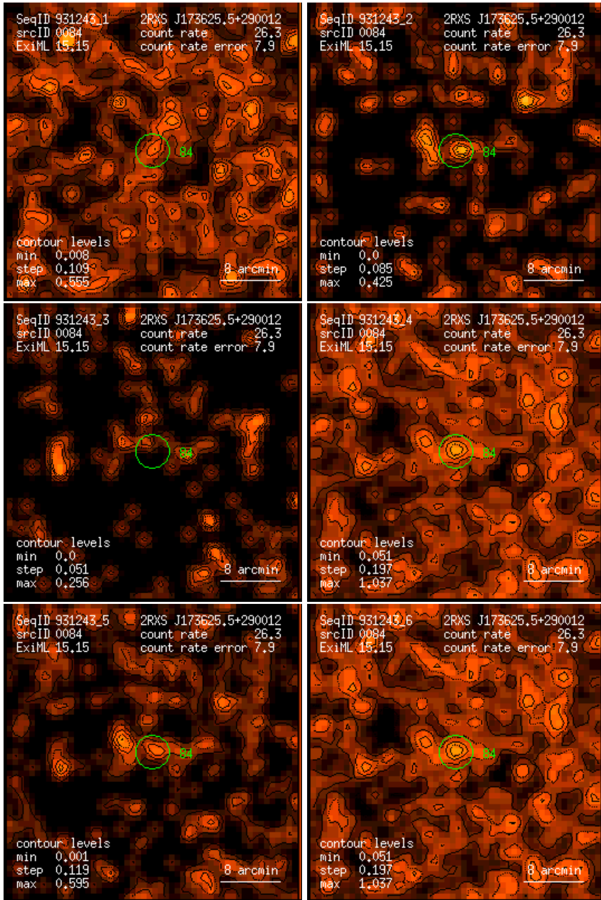
Figure 84: RASS 931243: detection 0084: band rate images, Gaussian filter: (1) PSPC channels 11 – 41, (2) 52 – 90, (3) 91 – 201, (4) 11 – 235, (5) 52 – 201, (6) 11 – 201. Broad band rates in counts/ks. Band rate contour levels in counts/ks/arcmin 2 .
