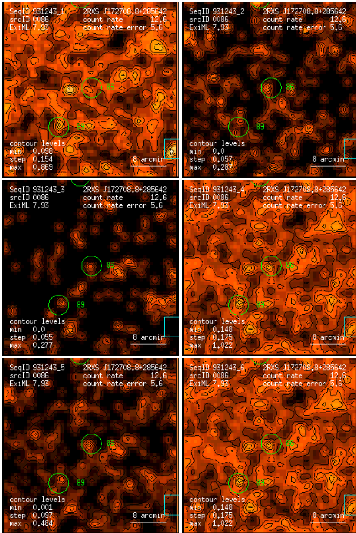
Figure 86: RASS 931243: detection 0086: band rate images, Gaussian filter: (1) PSPC channels 11 – 41, (2) 52 – 90, (3) 91 – 201, (4) 11 – 235, (5) 52 – 201, (6) 11 – 201. Broad band rates in counts/ks. Band rate contour levels in counts/ks/arcmin 2 .
