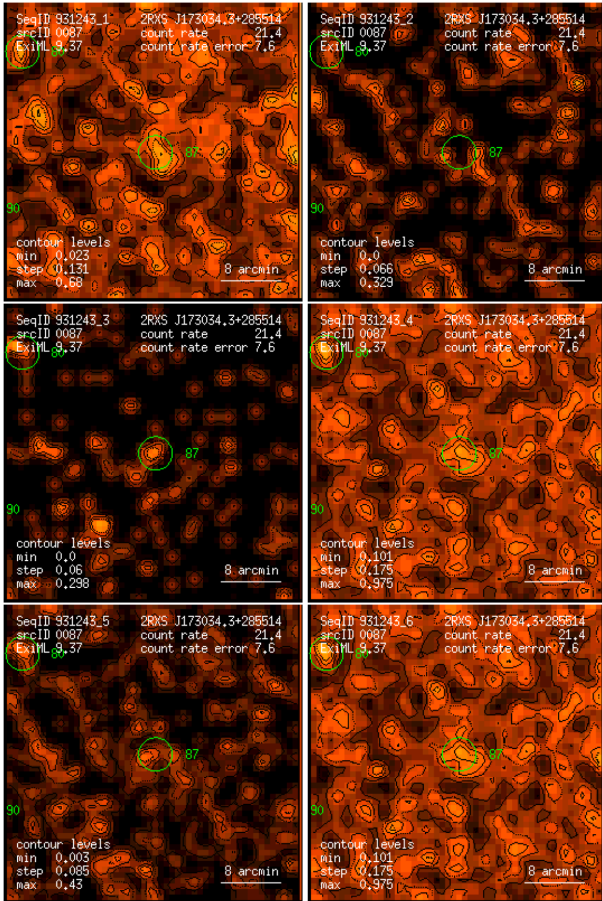
Figure 87: RASS 931243: detection 0087: band rate images, Gaussian filter: (1) PSPC channels 11 – 41, (2) 52 – 90, (3) 91 – 201, (4) 11 – 235, (5) 52 – 201, (6) 11 – 201. Broad band rates in counts/ks. Band rate contour levels in counts/ks/arcmin 2 .
