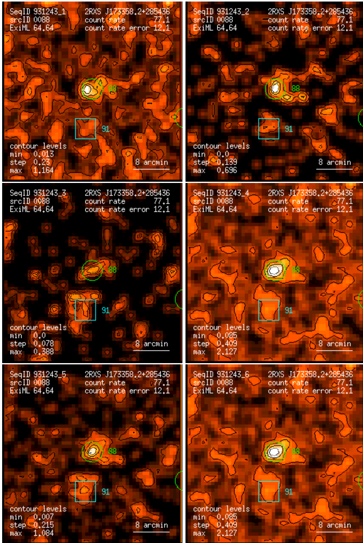
Figure 88: RASS 931243: detection 0088: band rate images, Gaussian filter: (1) PSPC channels 11 – 41, (2) 52 – 90, (3) 91 – 201, (4) 11 – 235, (5) 52 – 201, (6) 11 – 201. Broad band rates in counts/ks. Band rate contour levels in counts/ks/arcmin 2 .
