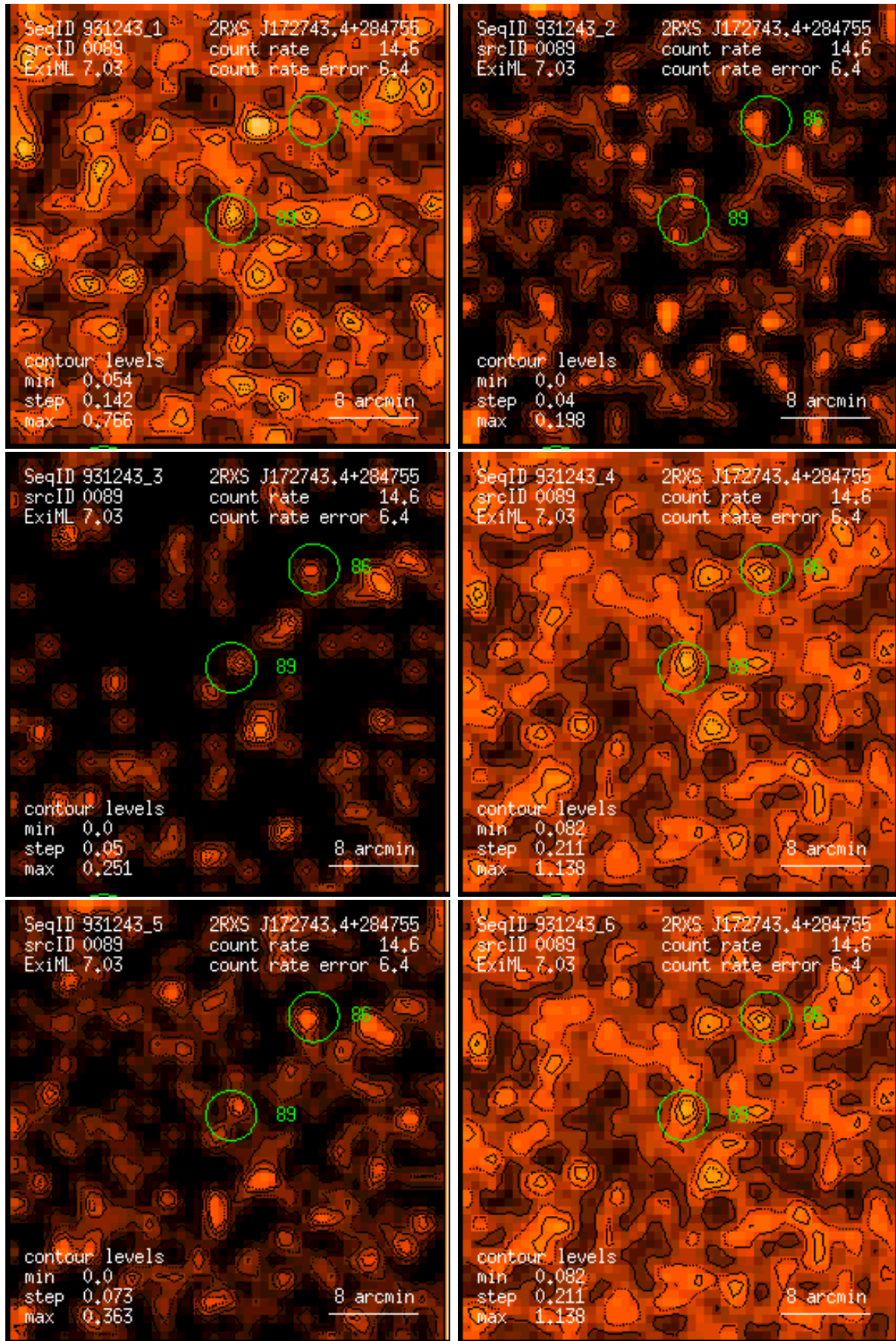
Figure 89: RASS 931243: detection 0089: band rate images, Gaussian filter: (1) PSPC channels 11 – 41, (2) 52 – 90, (3) 91 – 201, (4) 11 – 235, (5) 52 – 201, (6) 11 – 201. Broad band rates in counts/ks. Band rate contour levels in counts/ks/arcmin 2 .
