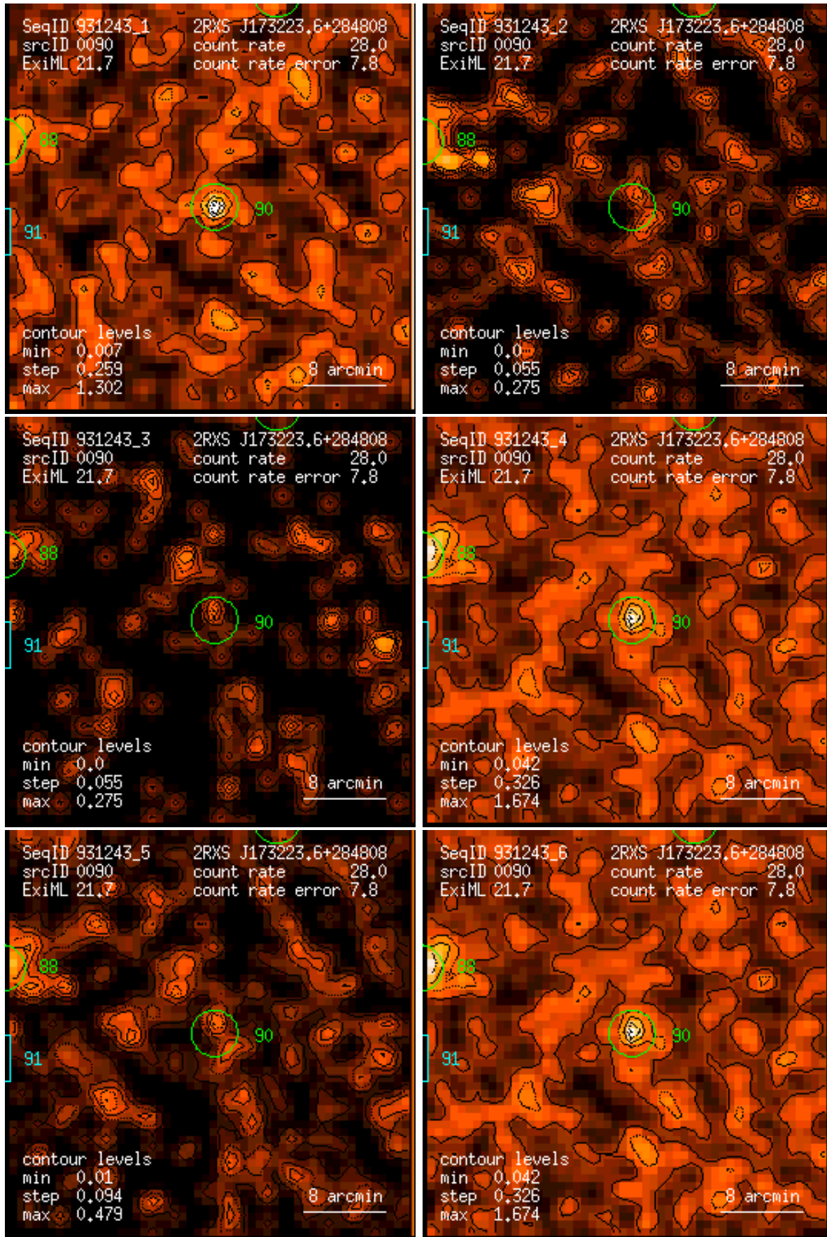
Figure 90: RASS 931243: detection 0090: band rate images, Gaussian filter: (1) PSPC channels 11 – 41, (2) 52 – 90, (3) 91 – 201, (4) 11 – 235, (5) 52 – 201, (6) 11 – 201. Broad band rates in counts/ks. Band rate contour levels in counts/ks/arcmin 2 .
