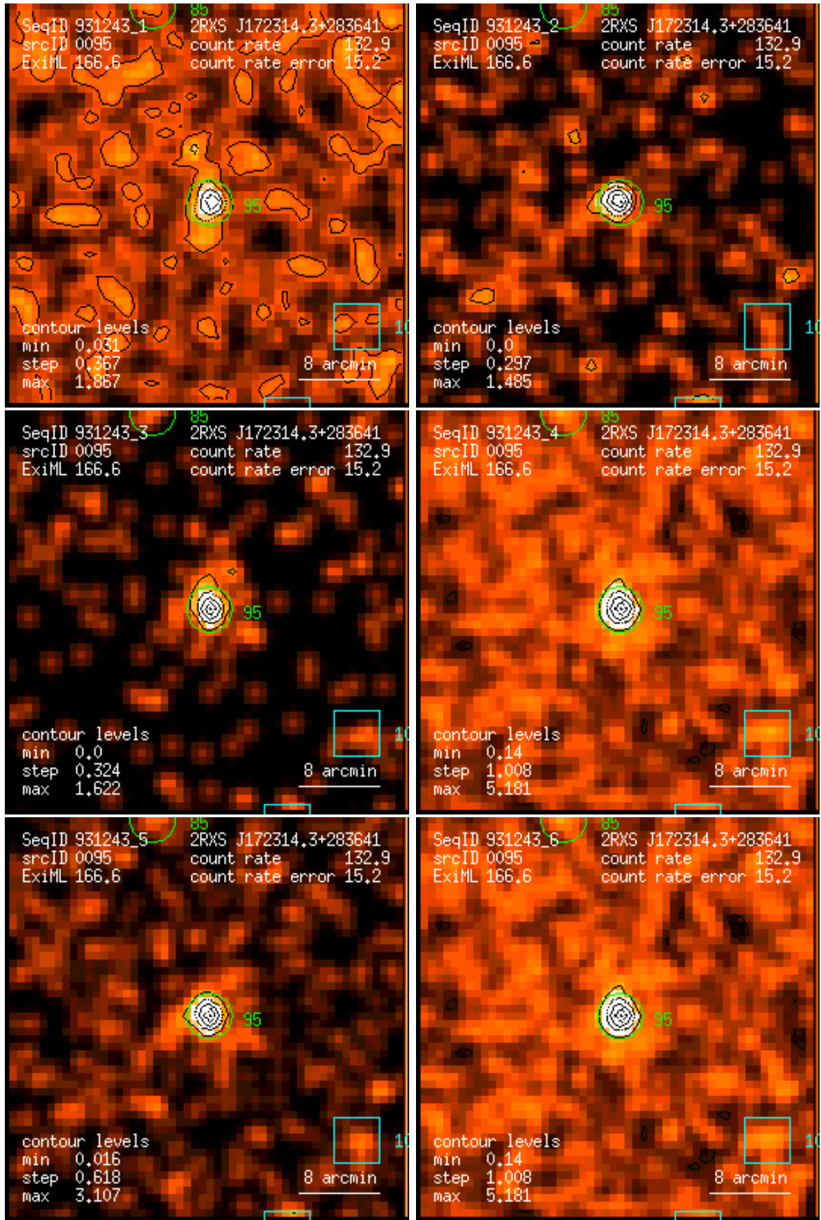
Figure 95: RASS 931243: detection 0095: band rate images, Gaussian filter: (1) PSPC channels 11 – 41, (2) 52 – 90, (3) 91 – 201, (4) 11 – 235, (5) 52 – 201, (6) 11 – 201. Broad band rates in counts/ks. Band rate contour levels in counts/ks/arcmin 2 .
