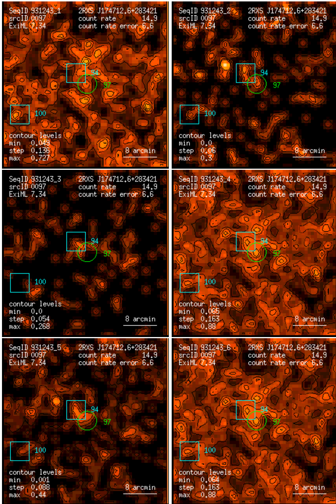
Figure 97: RASS 931243: detection 0097: band rate images, Gaussian filter: (1) PSPC channels 11 – 41, (2) 52 – 90, (3) 91 – 201, (4) 11 – 235, (5) 52 – 201, (6) 11 – 201. Broad band rates in counts/ks. Band rate contour levels in counts/ks/arcmin 2 .
