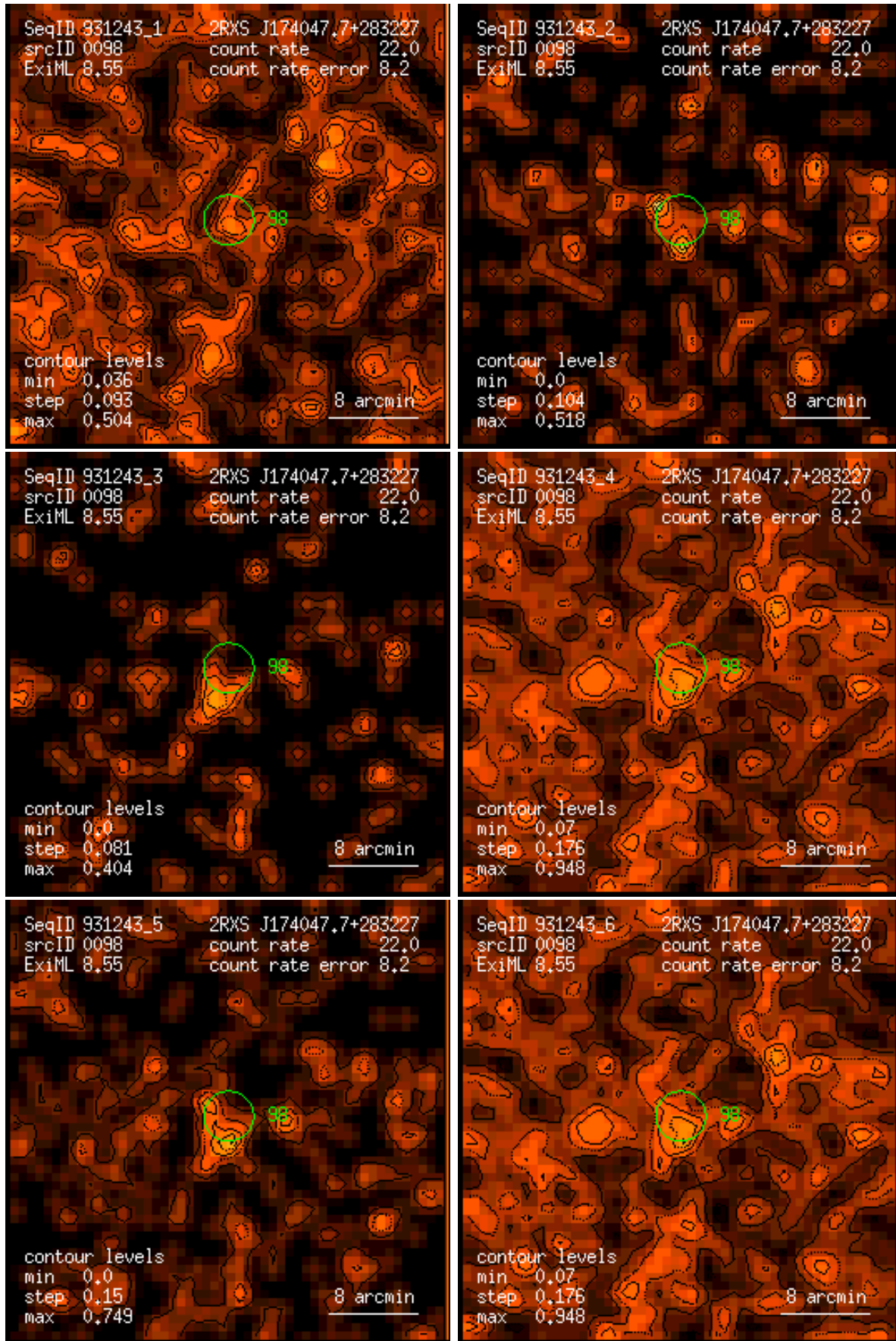
Figure 98: RASS 931243: detection 0098: band rate images, Gaussian filter: (1) PSPC channels 11 – 41, (2) 52 – 90, (3) 91 – 201, (4) 11 – 235, (5) 52 – 201, (6) 11 – 201. Broad band rates in counts/ks. Band rate contour levels in counts/ks/arcmin 2 .
