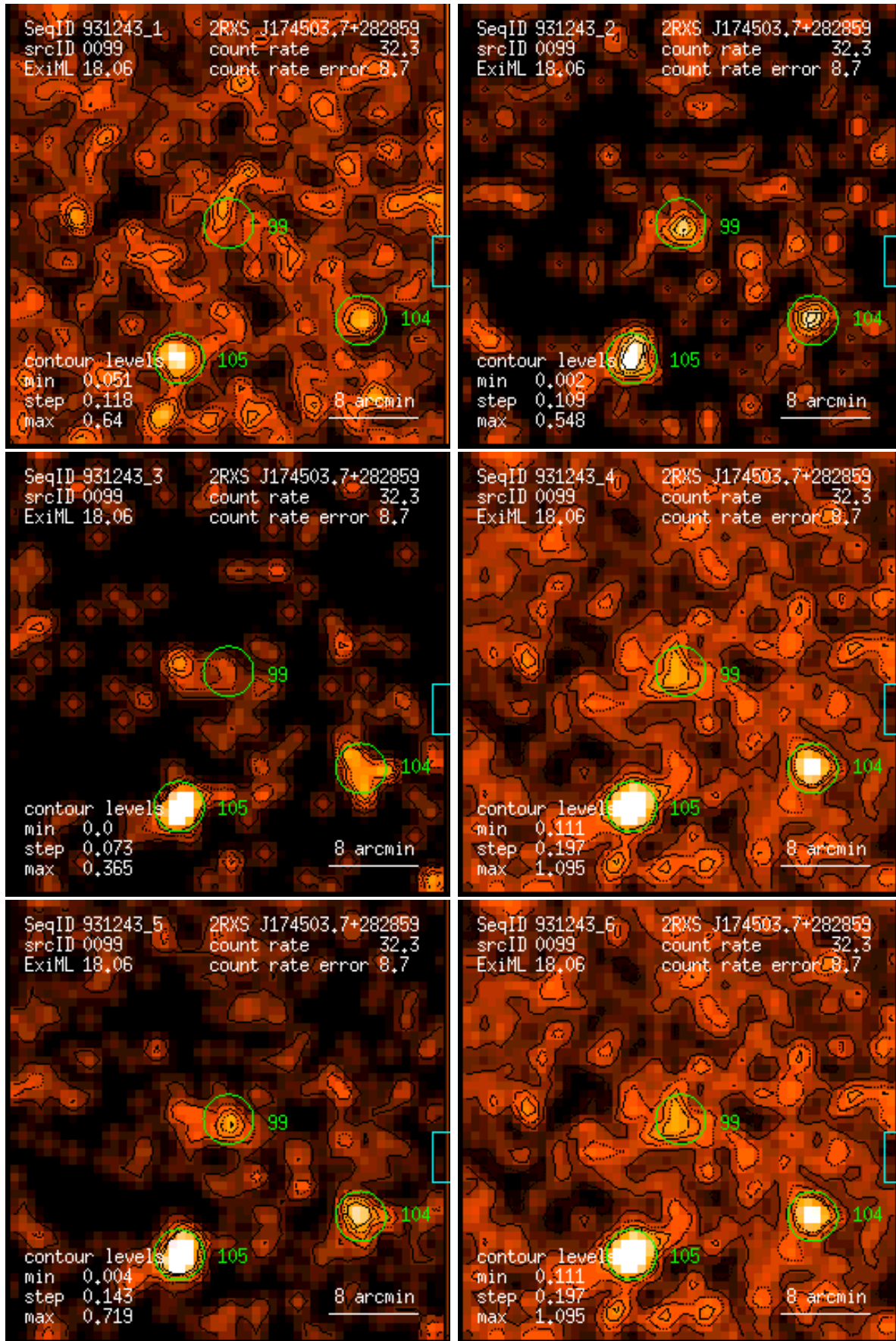
Figure 99: RASS 931243: detection 0099: band rate images, Gaussian filter: (1) PSPC channels 11 – 41, (2) 52 – 90, (3) 91 – 201, (4) 11 – 235, (5) 52 – 201, (6) 11 – 201. Broad band rates in counts/ks. Band rate contour levels in counts/ks/arcmin 2 .
