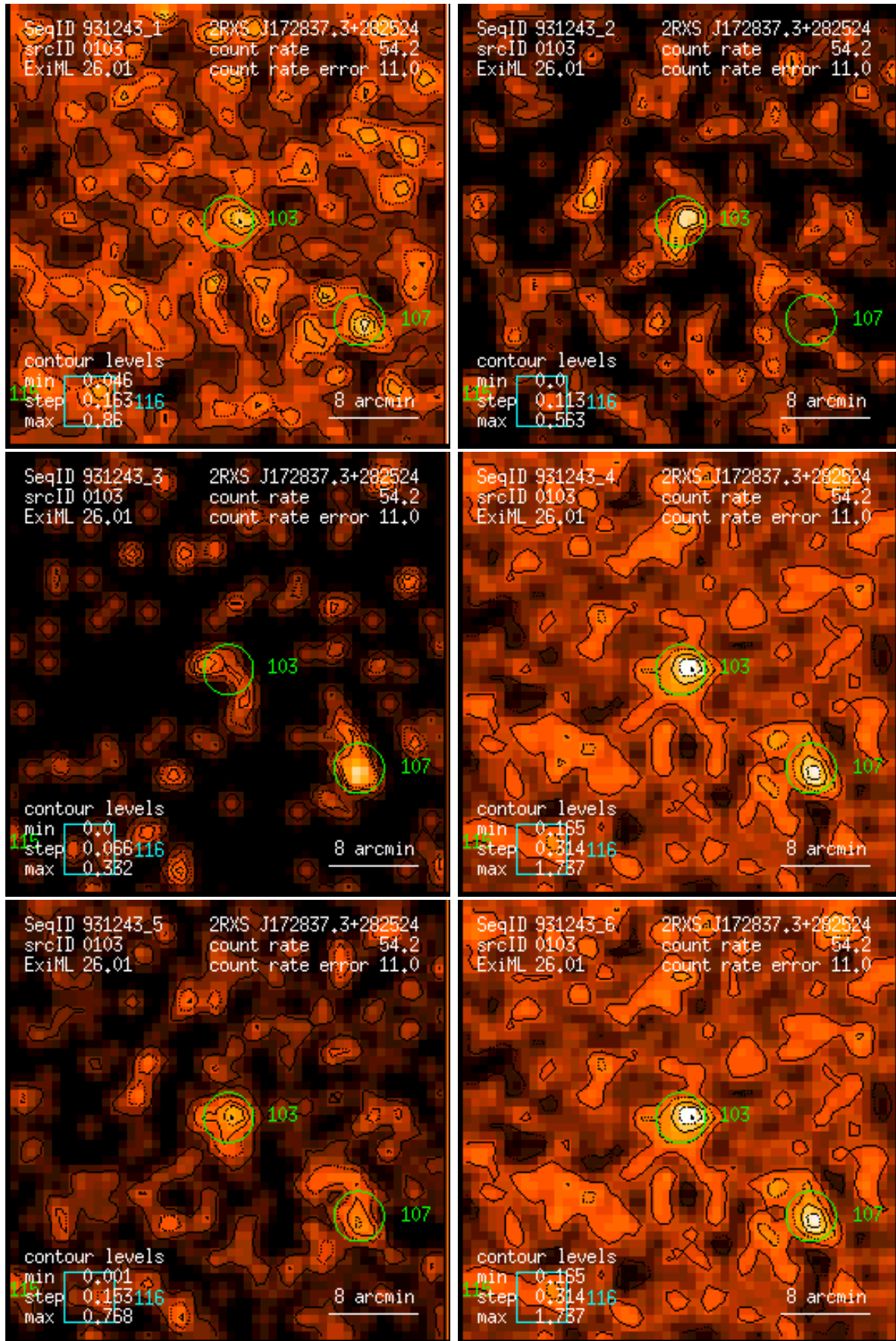
Figure 103: RASS 931243: detection 0103: band rate images, Gaussian filter: (1) PSPC channels 11 – 41, (2) 52 – 90, (3) 91 – 201, (4) 11 – 235, (5) 52 – 201, (6) 11 – 201. Broad band rates in counts/ks. Band rate contour levels in counts/ks/arcmin 2 .
