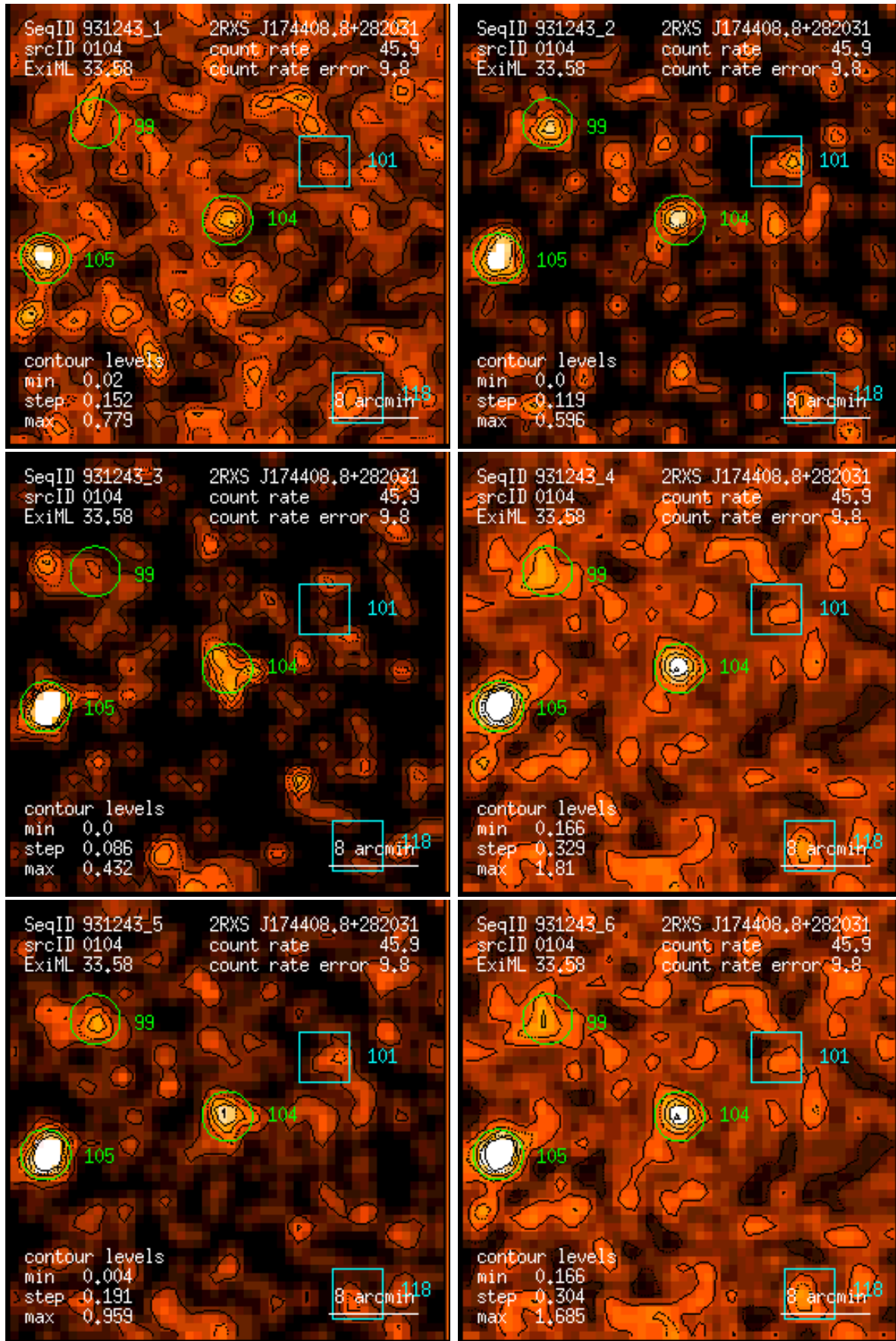
Figure 104: RASS 931243: detection 0104: band rate images, Gaussian filter: (1) PSPC channels 11 – 41, (2) 52 – 90, (3) 91 – 201, (4) 11 – 235, (5) 52 – 201, (6) 11 – 201. Broad band rates in counts/ks. Band rate contour levels in counts/ks/arcmin 2 .
