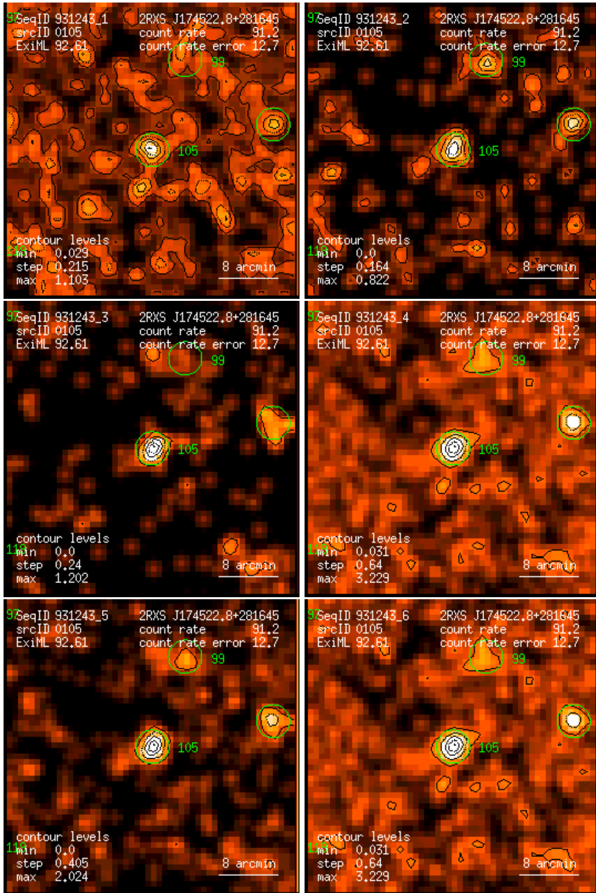
Figure 105: RASS 931243: detection 0105: band rate images, Gaussian filter: (1) PSPC channels 11 – 41, (2) 52 – 90, (3) 91 – 201, (4) 11 – 235, (5) 52 – 201, (6) 11 – 201. Broad band rates in counts/ks. Band rate contour levels in counts/ks/arcmin 2 .
