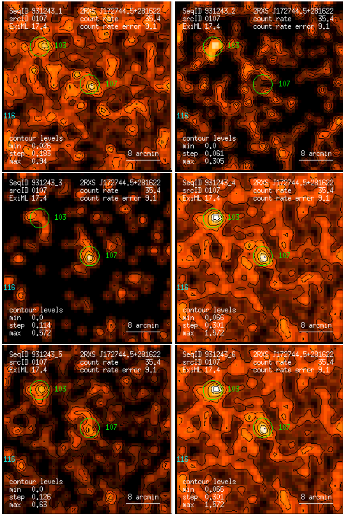
Figure 107: RASS 931243: detection 0107: band rate images, Gaussian filter: (1) PSPC channels 11 – 41, (2) 52 – 90, (3) 91 – 201, (4) 11 – 235, (5) 52 – 201, (6) 11 – 201. Broad band rates in counts/ks. Band rate contour levels in counts/ks/arcmin 2 .
