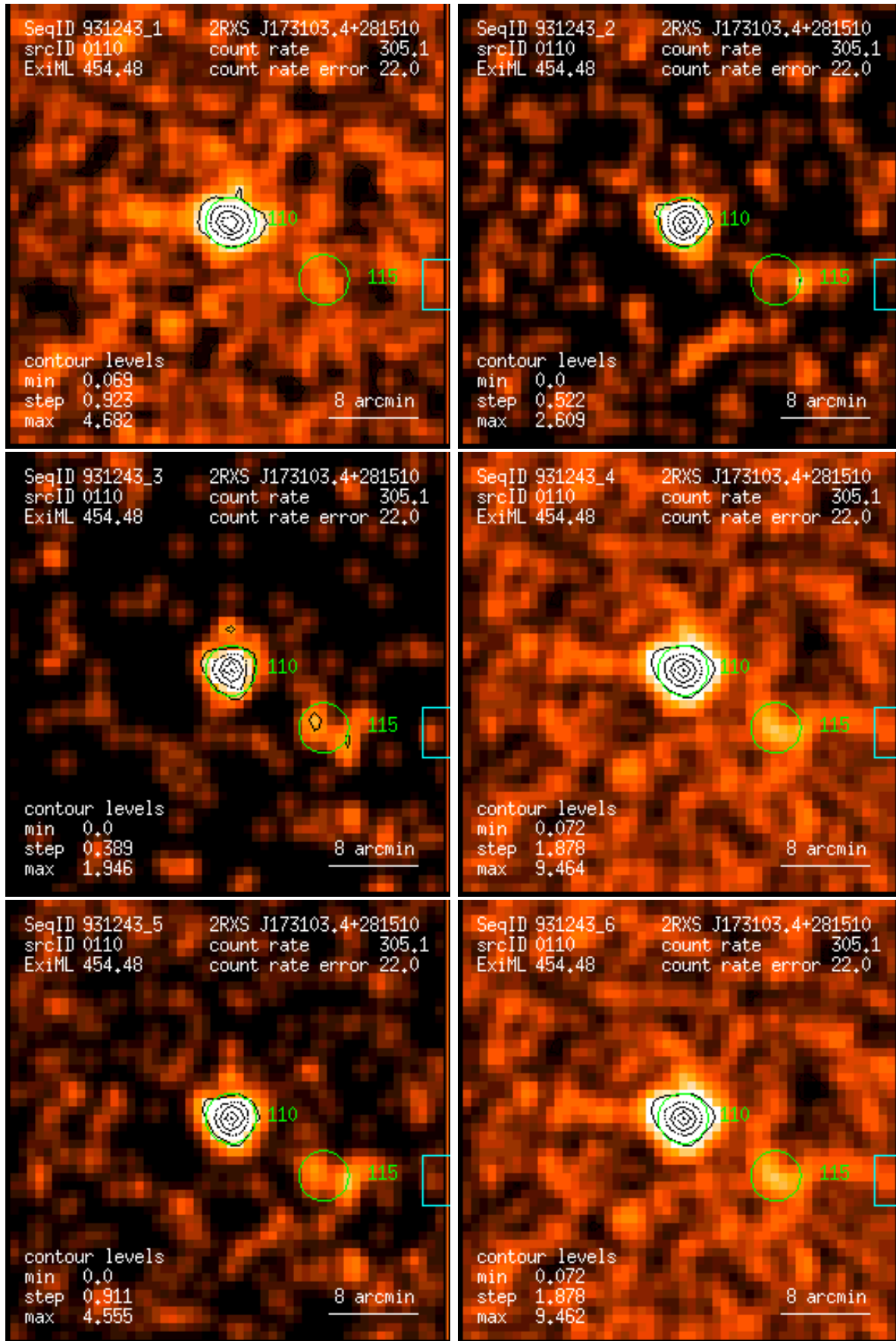
Figure 110: RASS 931243: detection 0110: band rate images, Gaussian filter: (1) PSPC channels 11 – 41, (2) 52 – 90, (3) 91 – 201, (4) 11 – 235, (5) 52 – 201, (6) 11 – 201. Broad band rates in counts/ks. Band rate contour levels in counts/ks/arcmin 2 .
