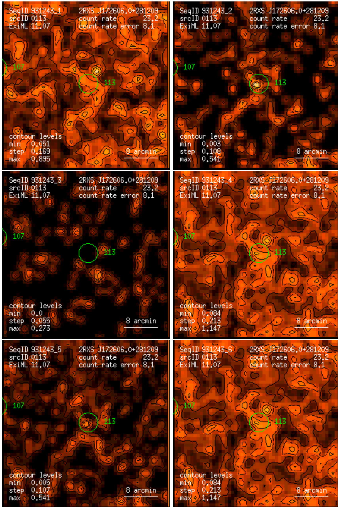
Figure 113: RASS 931243: detection 0113: band rate images, Gaussian filter: (1) PSPC channels 11 – 41, (2) 52 – 90, (3) 91 – 201, (4) 11 – 235, (5) 52 – 201, (6) 11 – 201. Broad band rates in counts/ks. Band rate contour levels in counts/ks/arcmin 2 .
