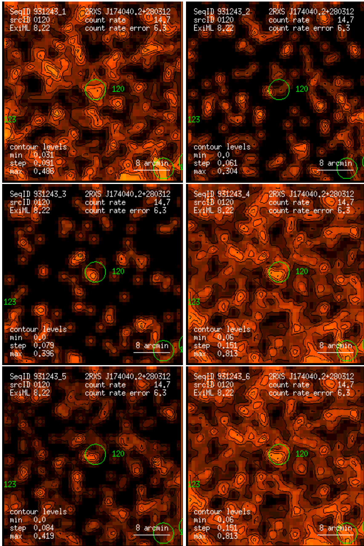
Figure 120: RASS 931243: detection 0120: band rate images, Gaussian filter: (1) PSPC channels 11 – 41, (2) 52 – 90, (3) 91 – 201, (4) 11 – 235, (5) 52 – 201, (6) 11 – 201. Broad band rates in counts/ks. Band rate contour levels in counts/ks/arcmin 2 .
