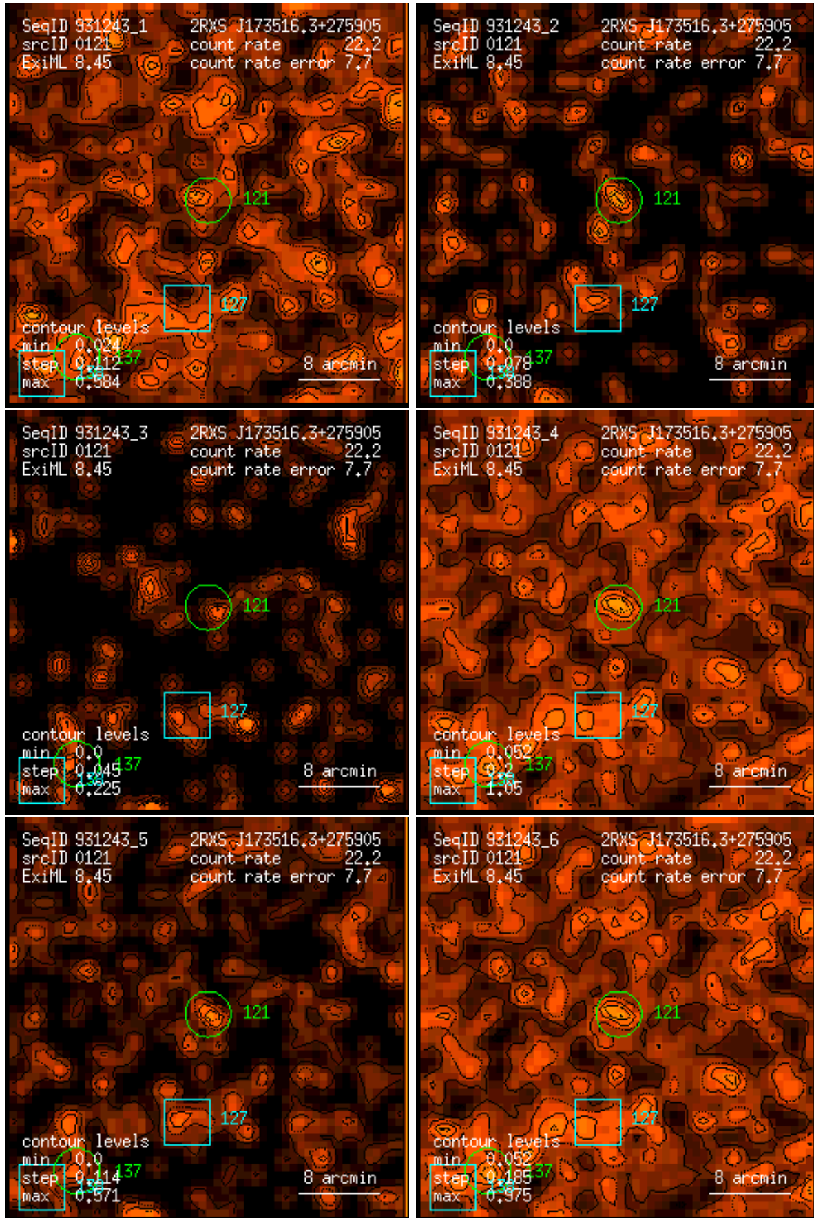
Figure 121: RASS 931243: detection 0121: band rate images, Gaussian filter: (1) PSPC channels 11 – 41, (2) 52 – 90, (3) 91 – 201, (4) 11 – 235, (5) 52 – 201, (6) 11 – 201. Broad band rates in counts/ks. Band rate contour levels in counts/ks/arcmin 2 .
