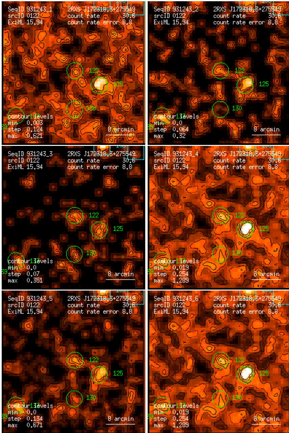
Figure 122: RASS 931243: detection 0122: band rate images, Gaussian filter: (1) PSPC channels 11 – 41, (2) 52 – 90, (3) 91 – 201, (4) 11 – 235, (5) 52 – 201, (6) 11 – 201. Broad band rates in counts/ks. Band rate contour levels in counts/ks/arcmin 2 .
