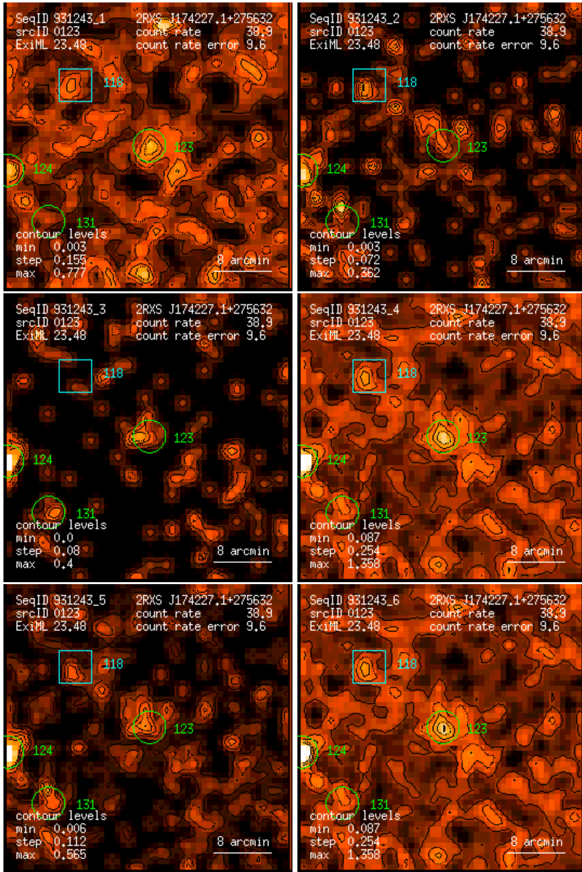
Figure 123: RASS 931243: detection 0123: band rate images, Gaussian filter: (1) PSPC channels 11 – 41, (2) 52 – 90, (3) 91 – 201, (4) 11 – 235, (5) 52 – 201, (6) 11 – 201. Broad band rates in counts/ks. Band rate contour levels in counts/ks/arcmin 2 .
