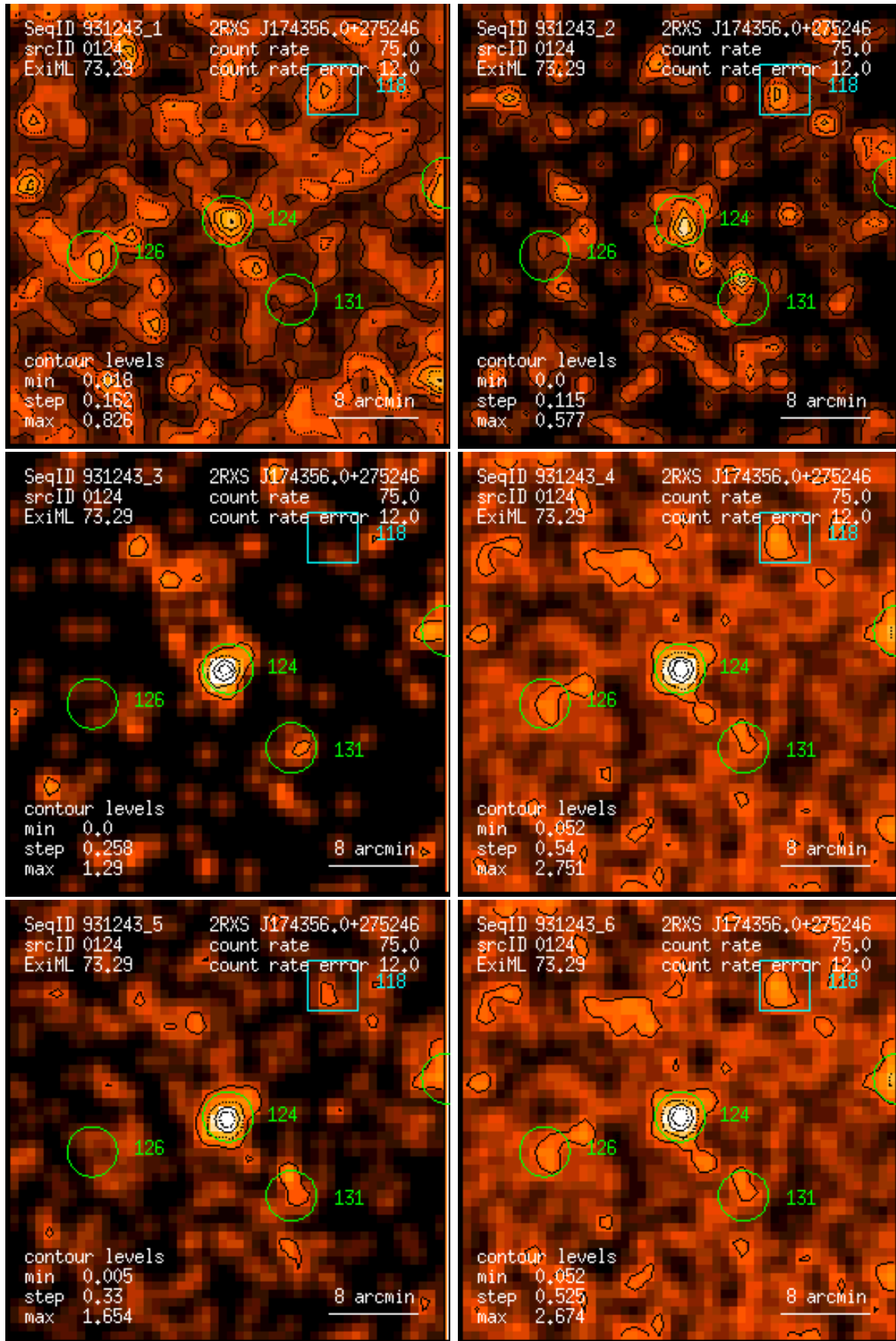
Figure 124: RASS 931243: detection 0124: band rate images, Gaussian filter: (1) PSPC channels 11 – 41, (2) 52 – 90, (3) 91 – 201, (4) 11 – 235, (5) 52 – 201, (6) 11 – 201. Broad band rates in counts/ks. Band rate contour levels in counts/ks/arcmin 2 .
