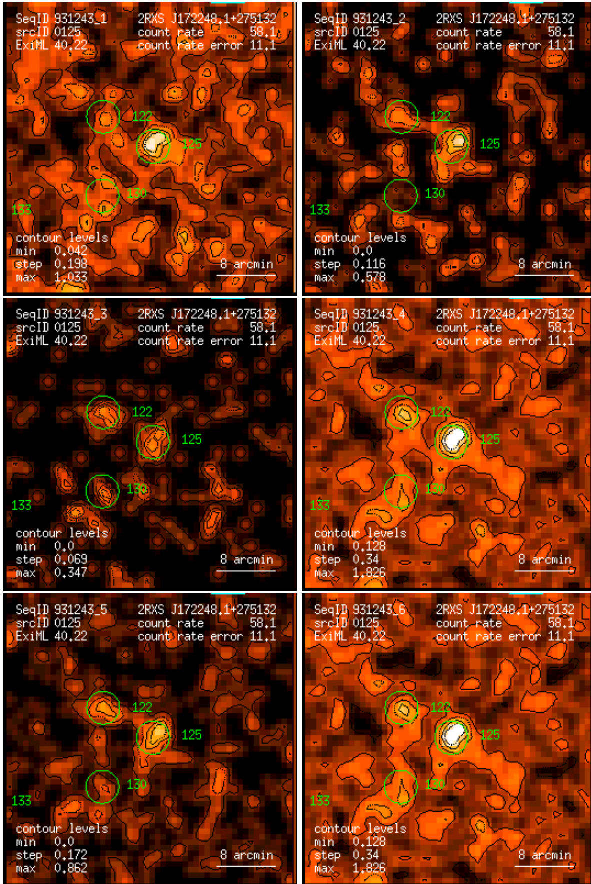
Figure 125: RASS 931243: detection 0125: band rate images, Gaussian filter: (1) PSPC channels 11 – 41, (2) 52 – 90, (3) 91 – 201, (4) 11 – 235, (5) 52 – 201, (6) 11 – 201. Broad band rates in counts/ks. Band rate contour levels in counts/ks/arcmin 2 .
