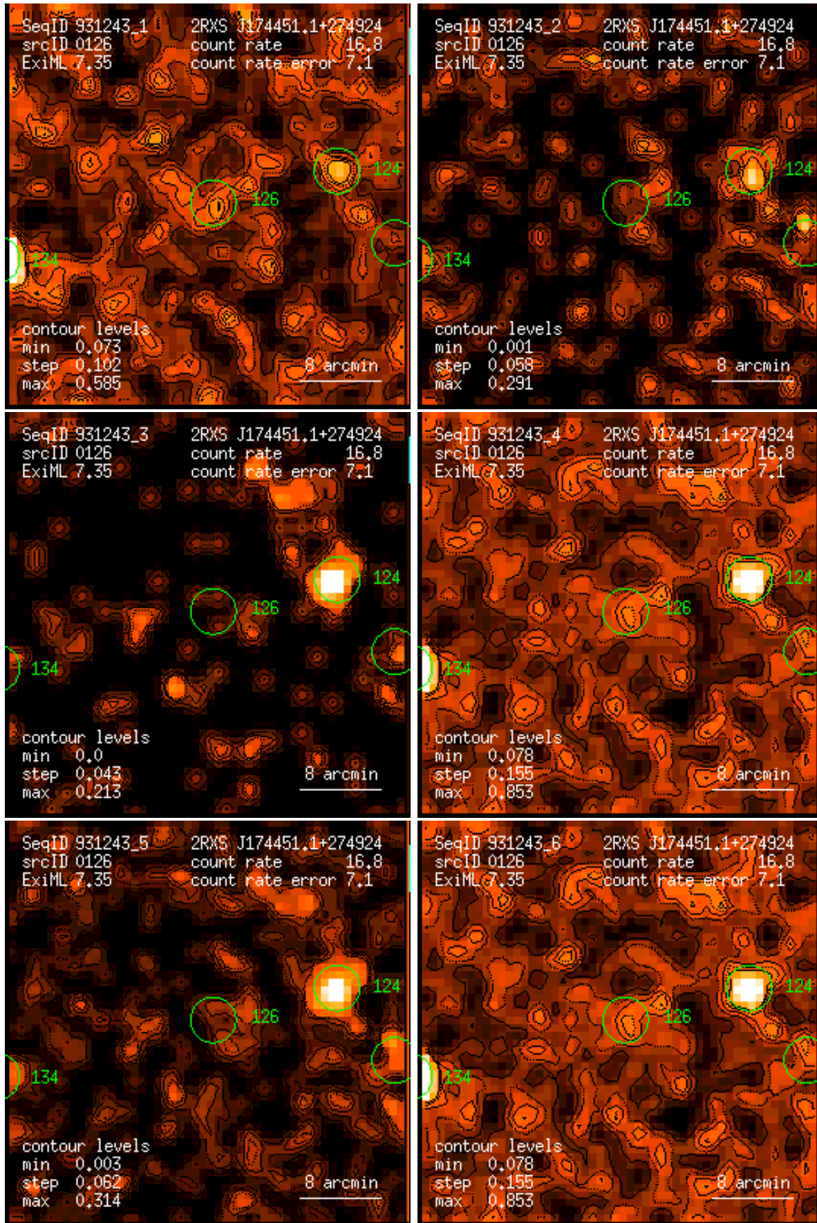
Figure 126: RASS 931243: detection 0126: band rate images, Gaussian filter: (1) PSPC channels 11 – 41, (2) 52 – 90, (3) 91 – 201, (4) 11 – 235, (5) 52 – 201, (6) 11 – 201. Broad band rates in counts/ks. Band rate contour levels in counts/ks/arcmin 2 .
