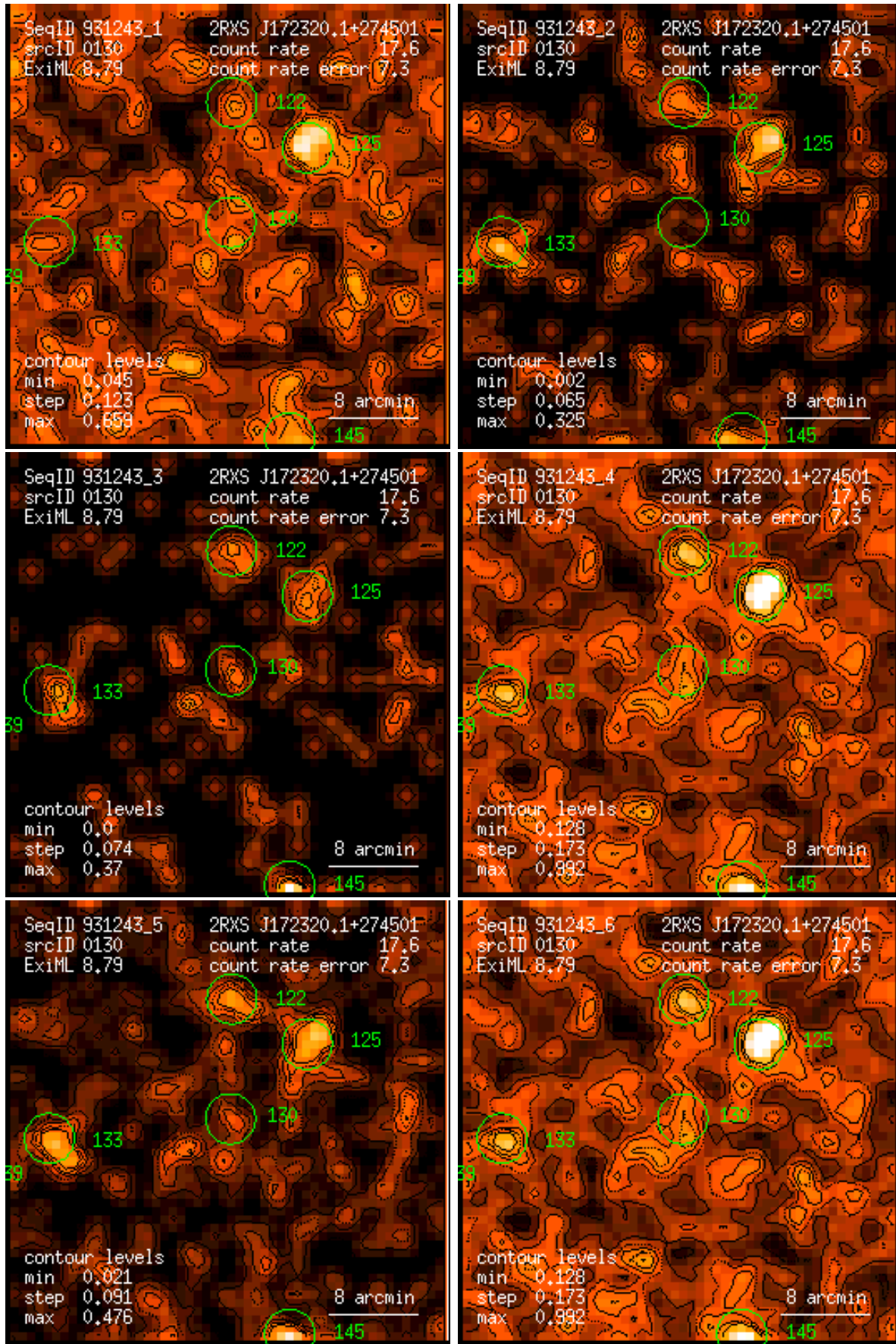
Figure 130: RASS 931243: detection 0130: band rate images, Gaussian filter: (1) PSPC channels 11 – 41, (2) 52 – 90, (3) 91 – 201, (4) 11 – 235, (5) 52 – 201, (6) 11 – 201. Broad band rates in counts/ks. Band rate contour levels in counts/ks/arcmin 2 .
