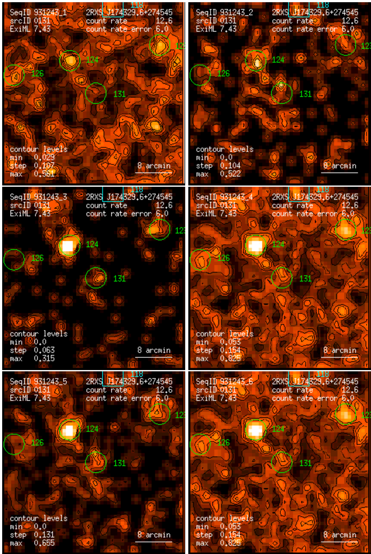
Figure 131: RASS 931243: detection 0131: band rate images, Gaussian filter: (1) PSPC channels 11 – 41, (2) 52 – 90, (3) 91 – 201, (4) 11 – 235, (5) 52 – 201, (6) 11 – 201. Broad band rates in counts/ks. Band rate contour levels in counts/ks/arcmin 2 .
