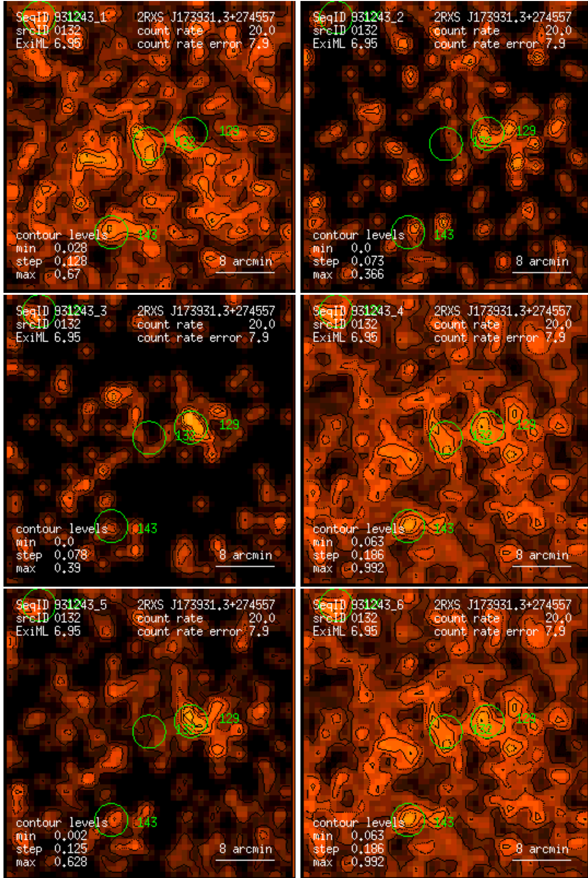
Figure 132: RASS 931243: detection 0132: band rate images, Gaussian filter: (1) PSPC channels 11 – 41, (2) 52 – 90, (3) 91 – 201, (4) 11 – 235, (5) 52 – 201, (6) 11 – 201. Broad band rates in counts/ks. Band rate contour levels in counts/ks/arcmin 2 .
