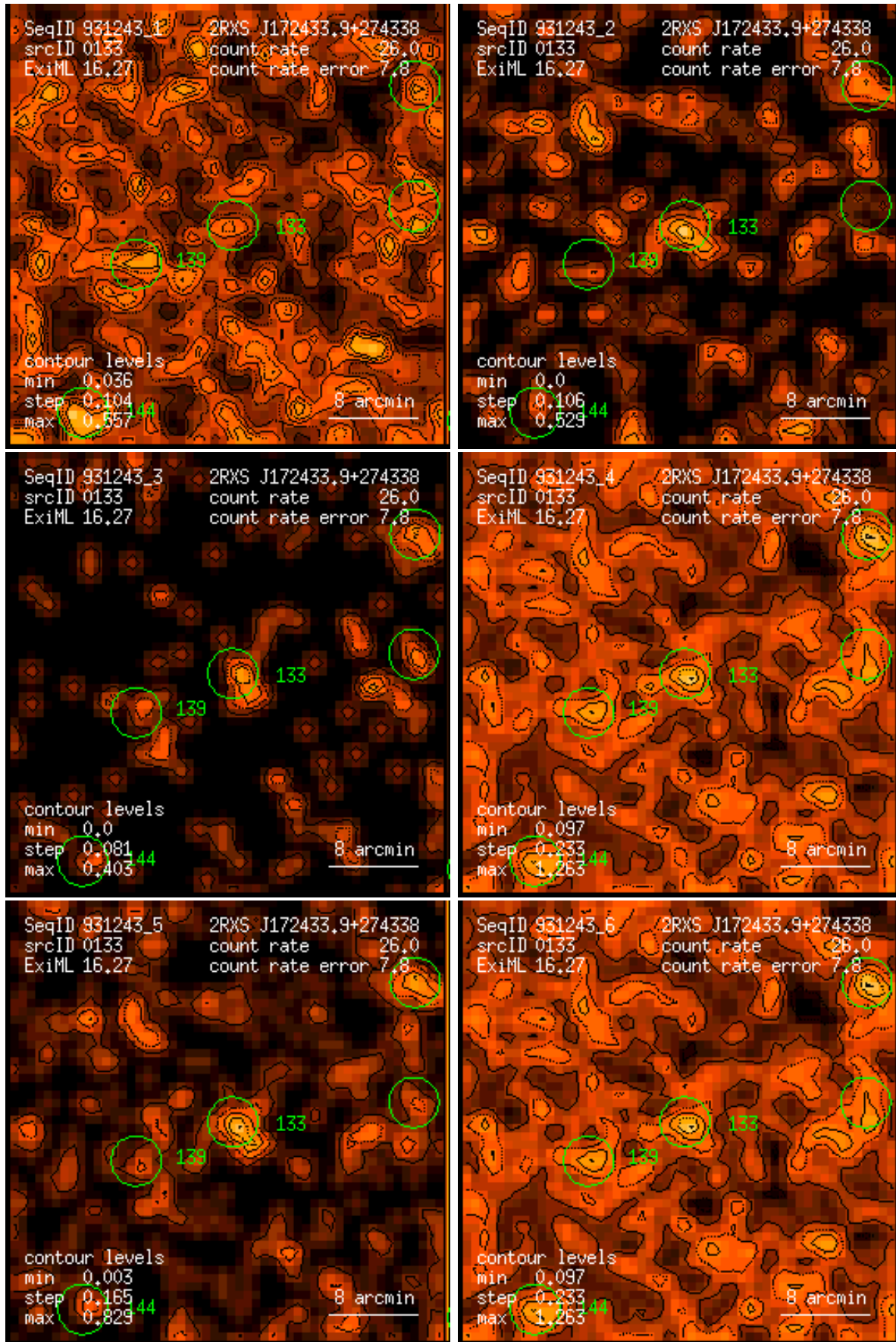
Figure 133: RASS 931243: detection 0133: band rate images, Gaussian filter: (1) PSPC channels 11 – 41, (2) 52 – 90, (3) 91 – 201, (4) 11 – 235, (5) 52 – 201, (6) 11 – 201. Broad band rates in counts/ks. Band rate contour levels in counts/ks/arcmin 2 .
