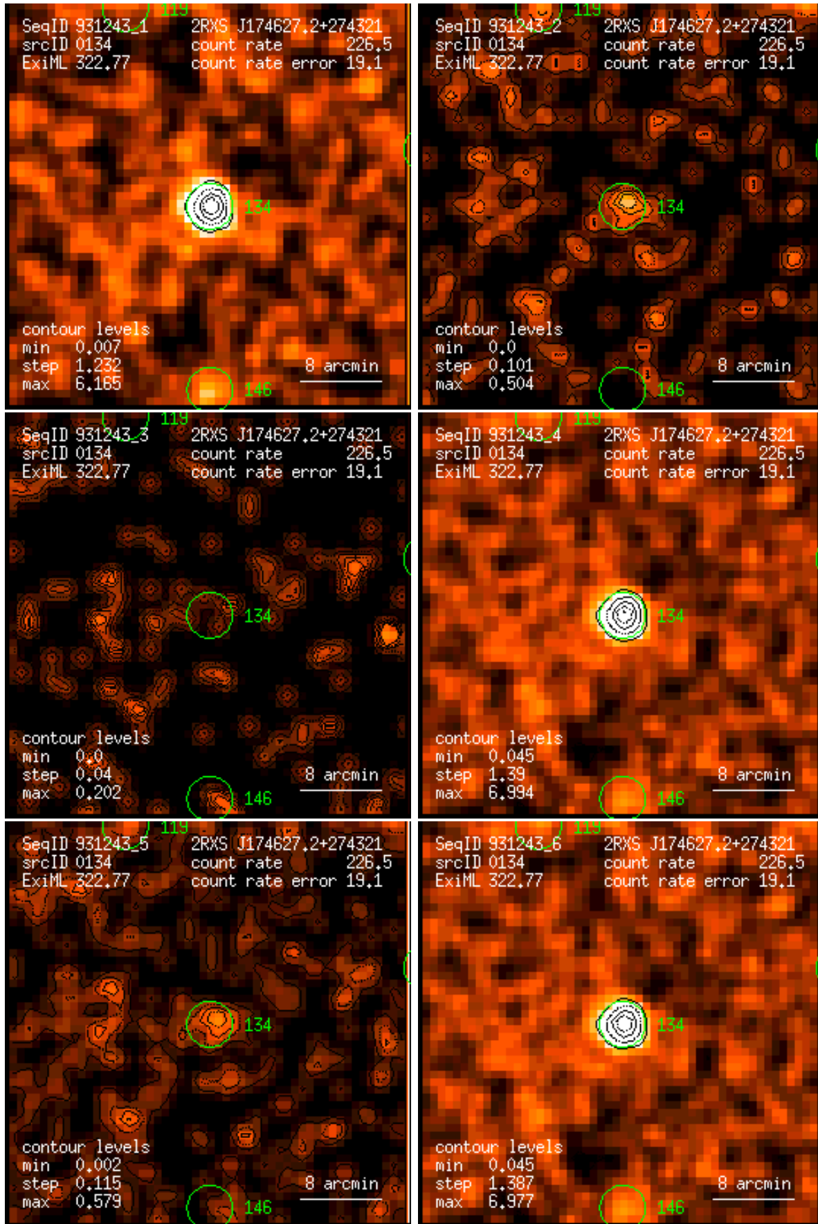
Figure 134: RASS 931243: detection 0134: band rate images, Gaussian filter: (1) PSPC channels 11 – 41, (2) 52 – 90, (3) 91 – 201, (4) 11 – 235, (5) 52 – 201, (6) 11 – 201. Broad band rates in counts/ks. Band rate contour levels in counts/ks/arcmin 2 .
