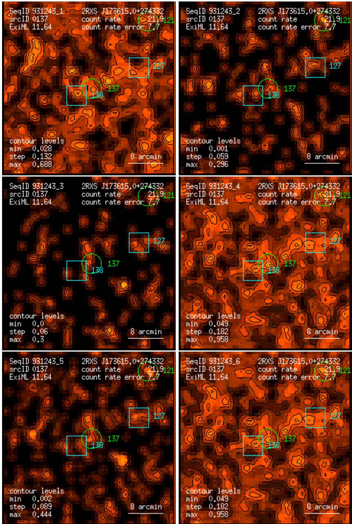
Figure 137: RASS 931243: detection 0137: band rate images, Gaussian filter: (1) PSPC channels 11 – 41, (2) 52 – 90, (3) 91 – 201, (4) 11 – 235, (5) 52 – 201, (6) 11 – 201. Broad band rates in counts/ks. Band rate contour levels in counts/ks/arcmin 2 .
