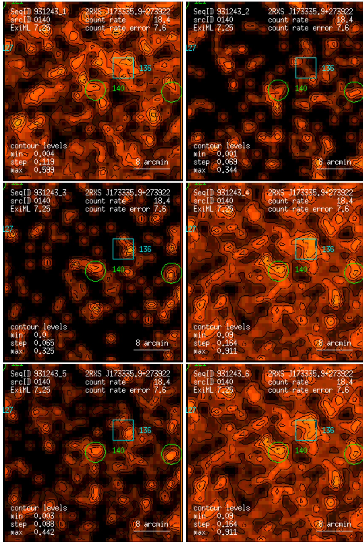
Figure 140: RASS 931243: detection 0140: band rate images, Gaussian filter: (1) PSPC channels 11 – 41, (2) 52 – 90, (3) 91 – 201, (4) 11 – 235, (5) 52 – 201, (6) 11 – 201. Broad band rates in counts/ks. Band rate contour levels in counts/ks/arcmin 2 .
