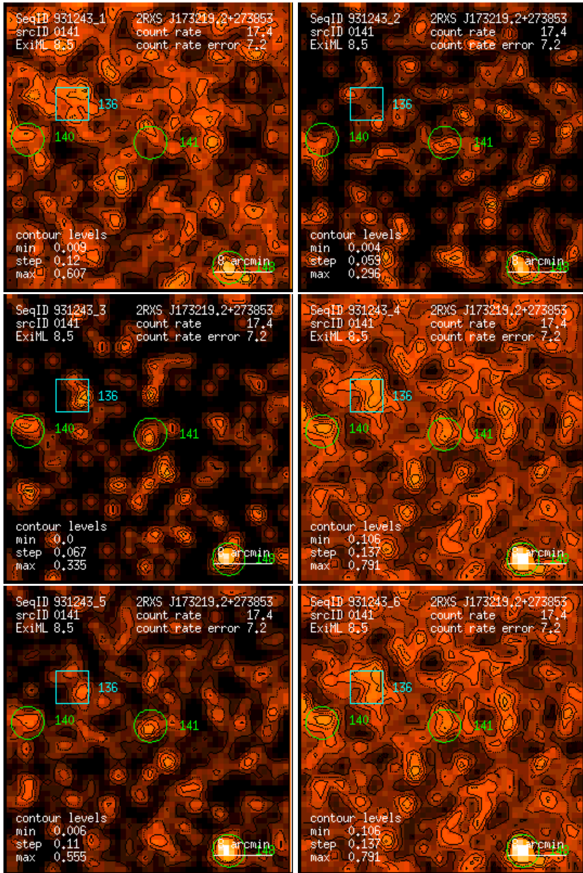
Figure 141: RASS 931243: detection 0141: band rate images, Gaussian filter: (1) PSPC channels 11 – 41, (2) 52 – 90, (3) 91 – 201, (4) 11 – 235, (5) 52 – 201, (6) 11 – 201. Broad band rates in counts/ks. Band rate contour levels in counts/ks/arcmin 2 .
