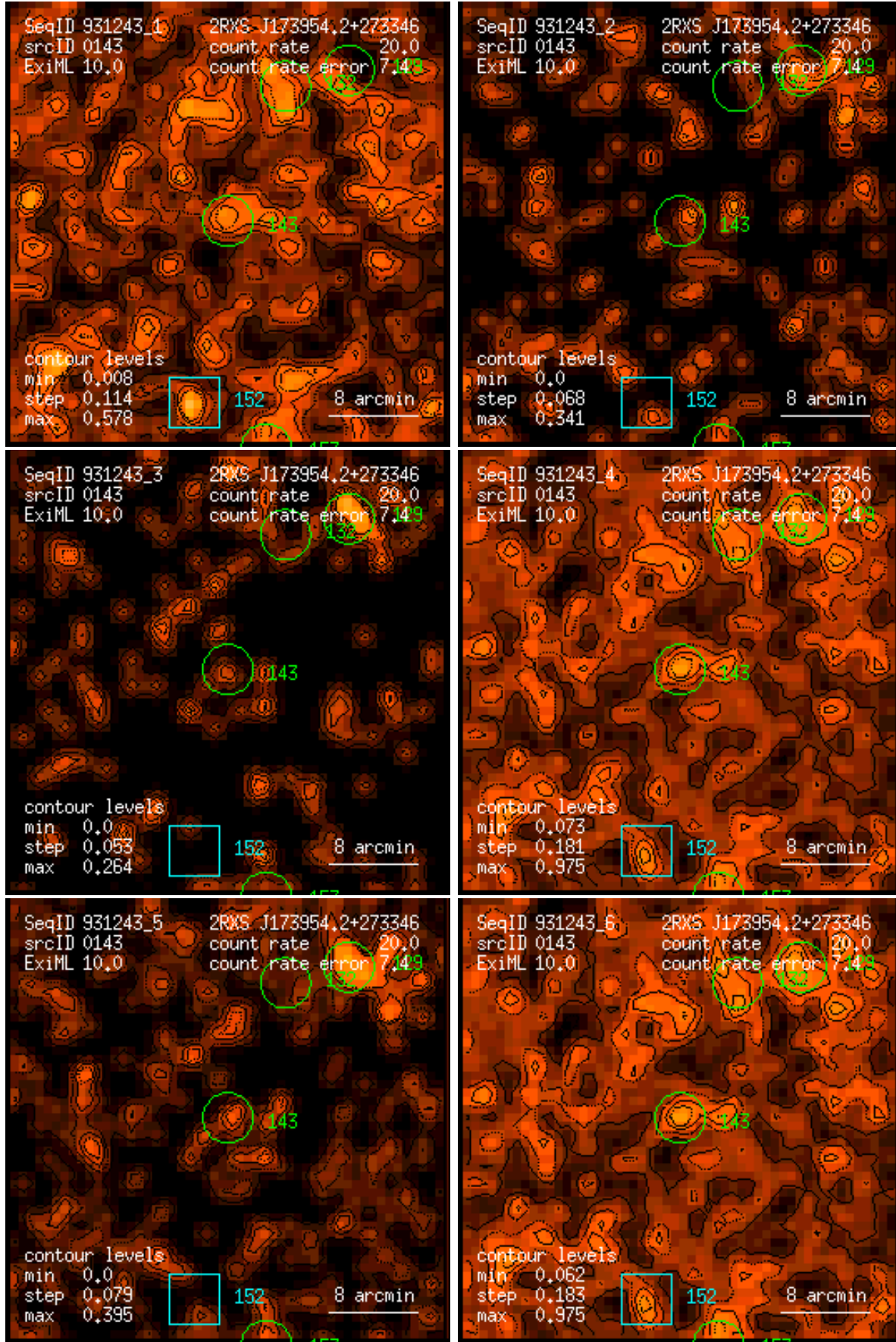
Figure 143: RASS 931243: detection 0143: band rate images, Gaussian filter: (1) PSPC channels 11 – 41, (2) 52 – 90, (3) 91 – 201, (4) 11 – 235, (5) 52 – 201, (6) 11 – 201. Broad band rates in counts/ks. Band rate contour levels in counts/ks/arcmin 2 .
