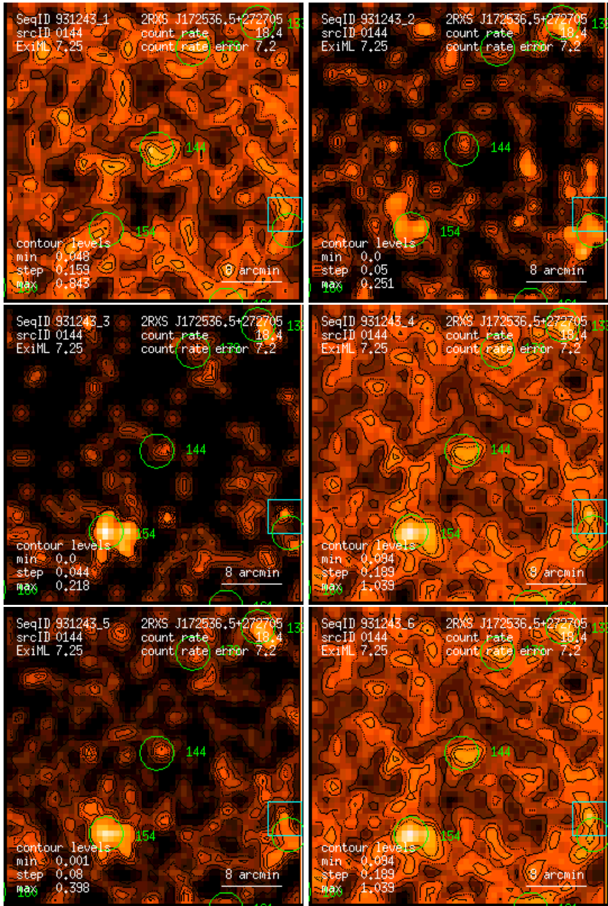
Figure 144: RASS 931243: detection 0144: band rate images, Gaussian filter: (1) PSPC channels 11 – 41, (2) 52 – 90, (3) 91 – 201, (4) 11 – 235, (5) 52 – 201, (6) 11 – 201. Broad band rates in counts/ks. Band rate contour levels in counts/ks/arcmin 2 .
